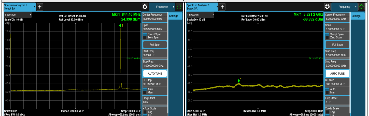
CH 20625 (846.5 MHz)
