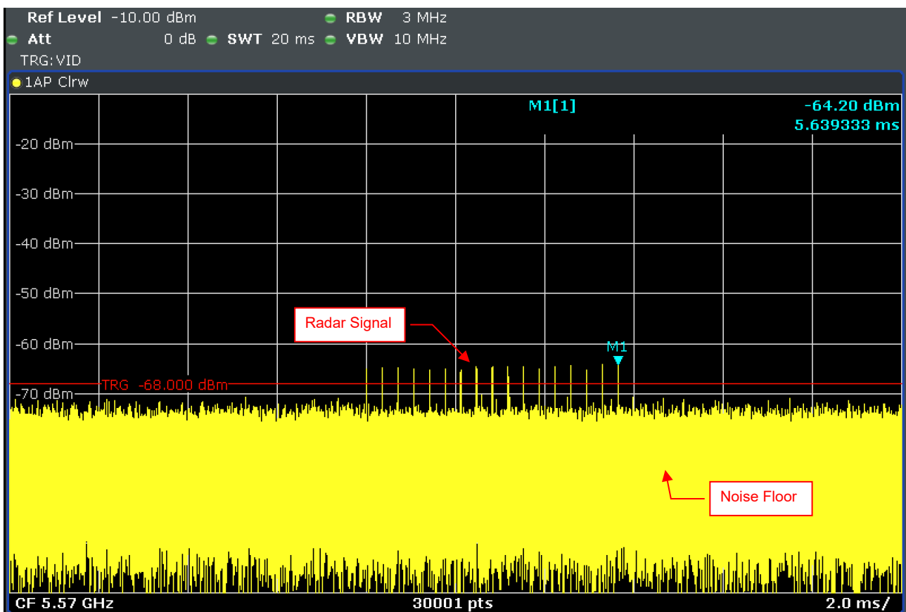
Radar Signal 3
