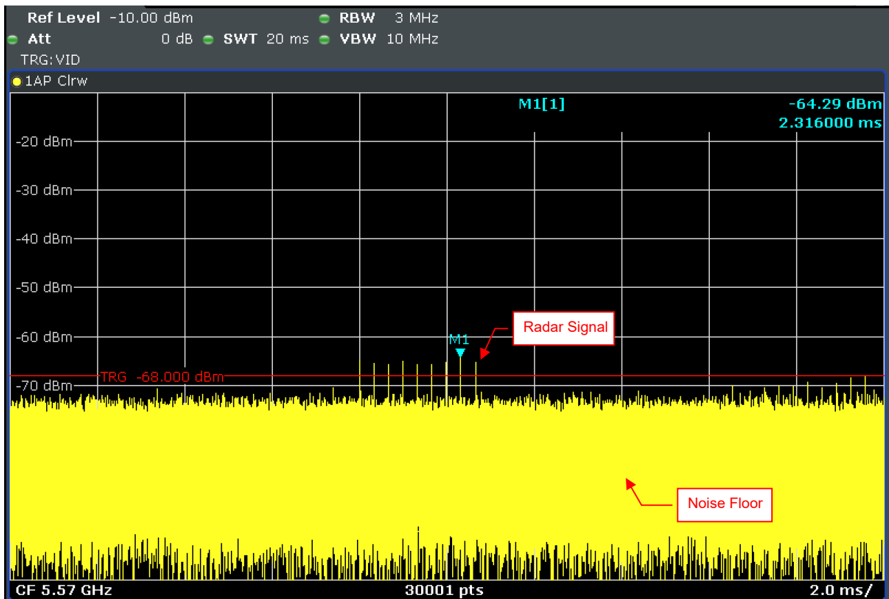
Radar Signal 6
