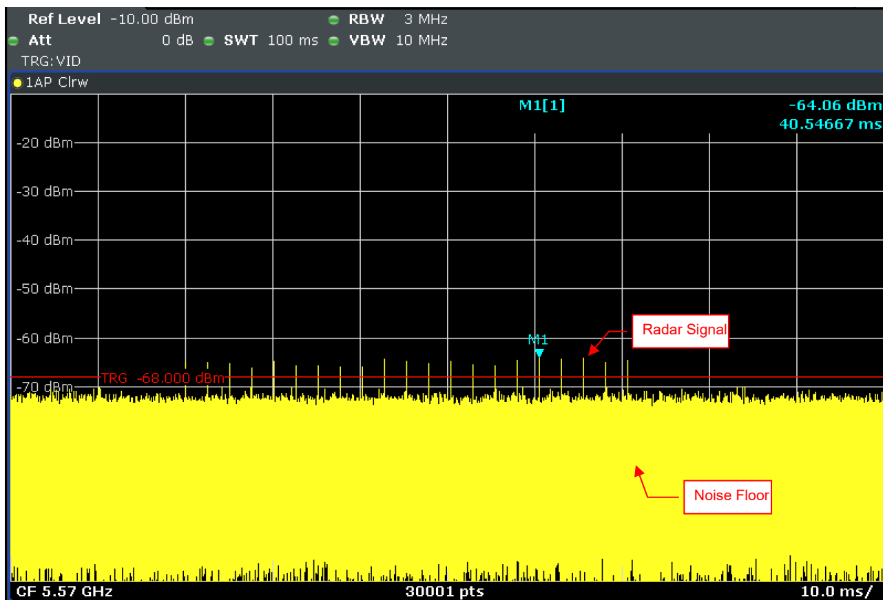
Radar Signal 1 (Test B)
