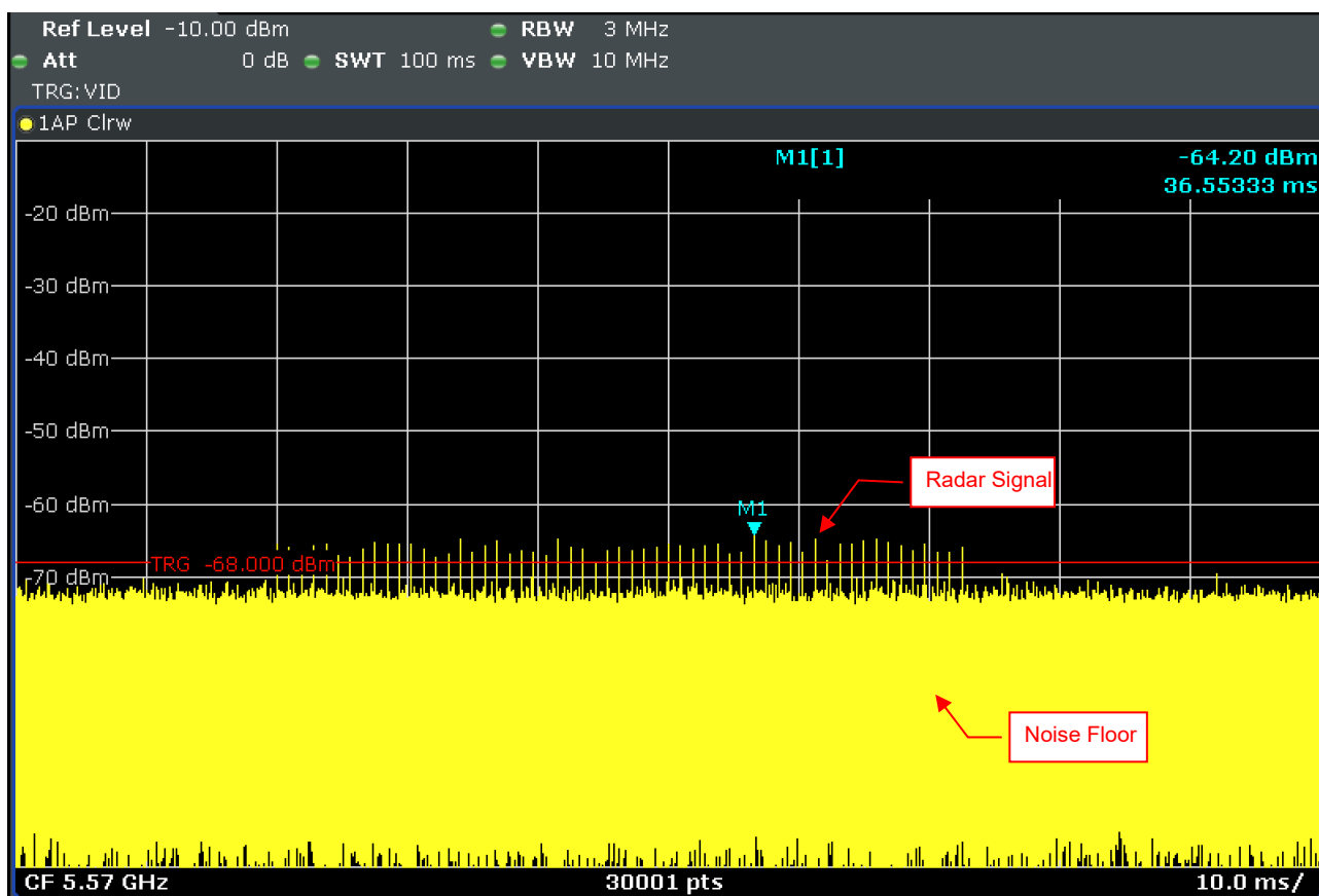
Radar Signal 1 (Test A)
