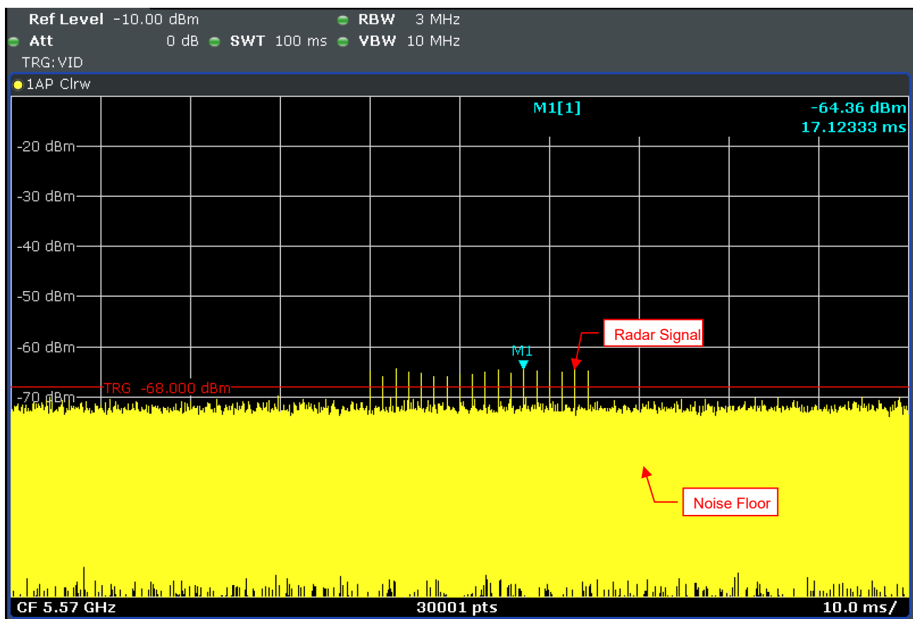
Radar Signal 0
