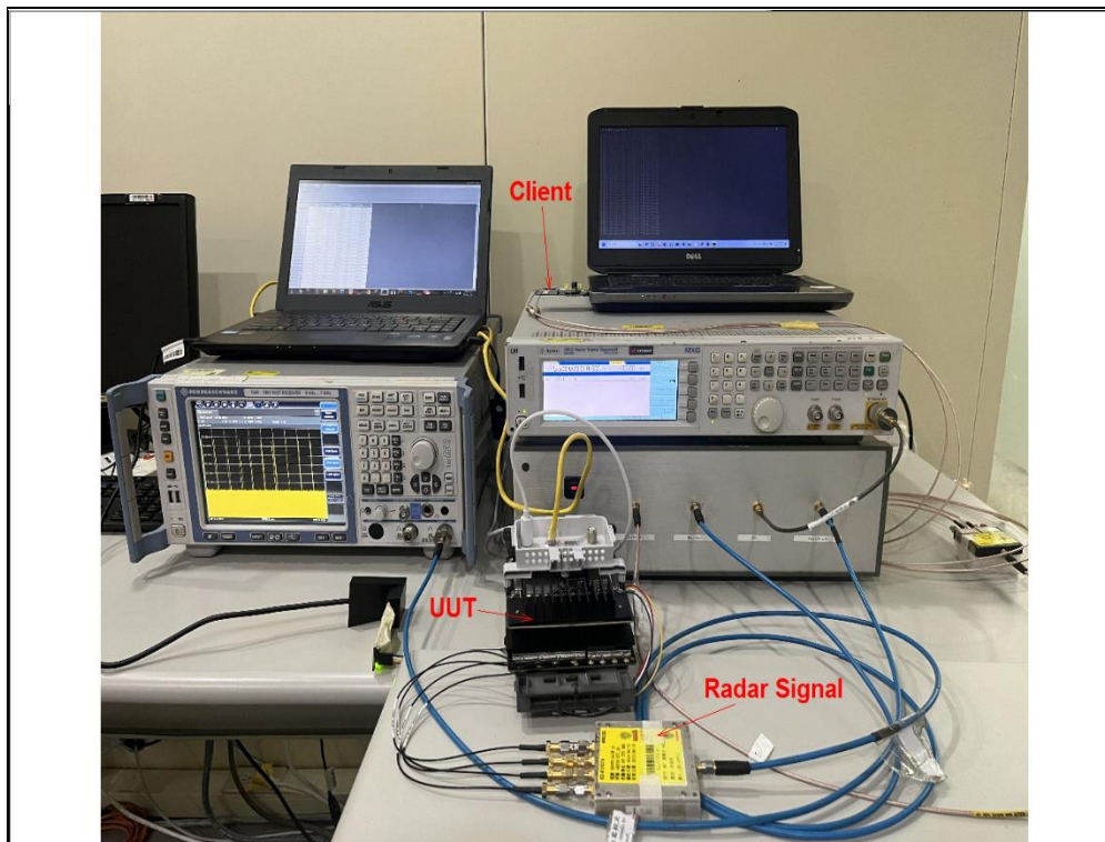
Setup Photo
