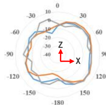
ZX-Cut
