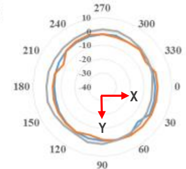
XY-Cut
