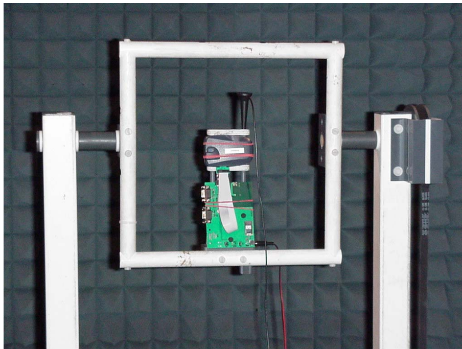
Picture 1 : Test setup for radiated measurements
