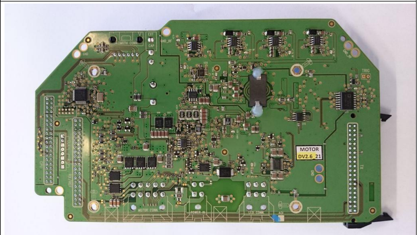
HALO PSU PCBA
