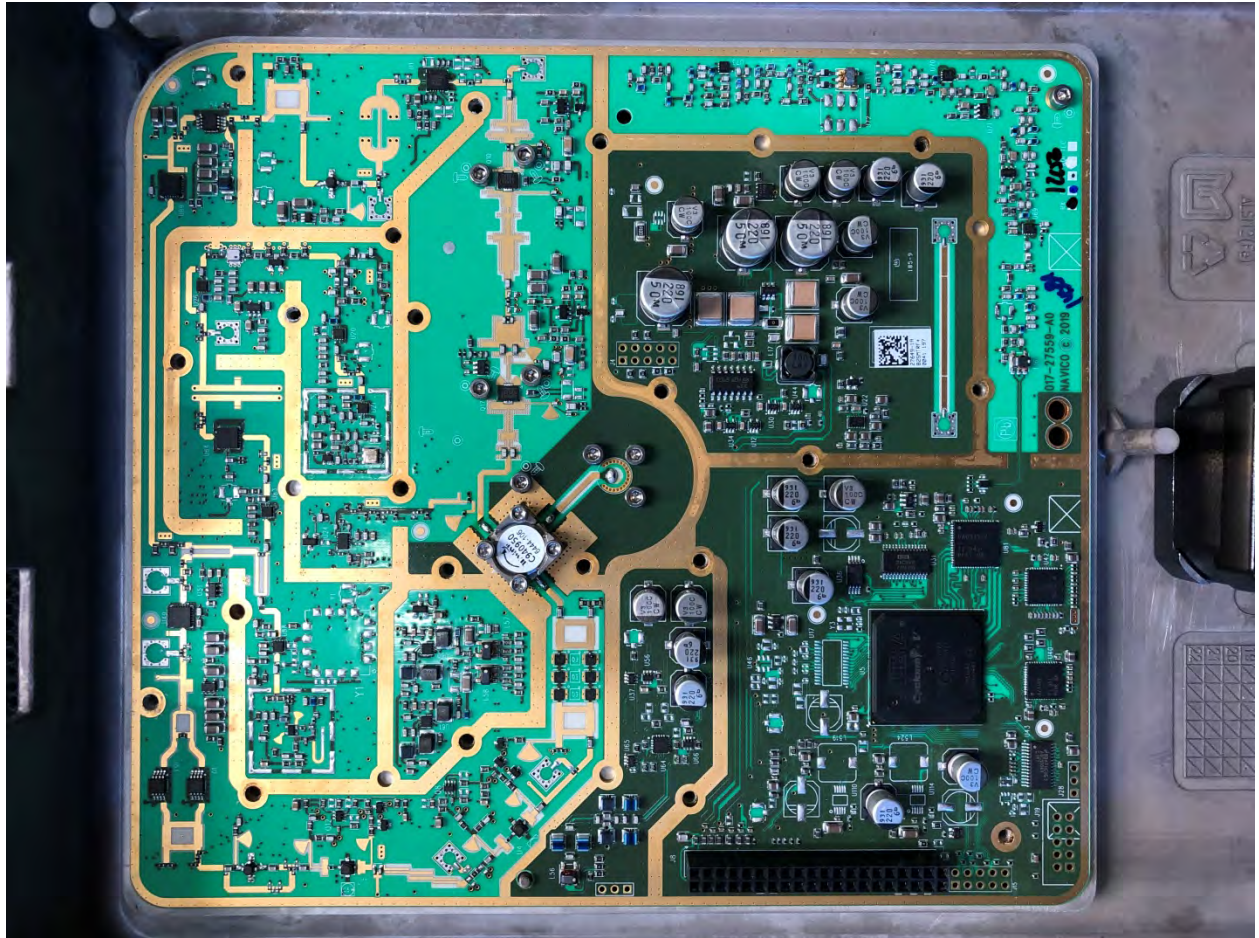
RF PCB
