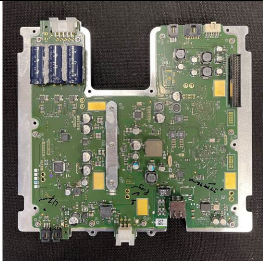
CPU PCBA – assembly on plate
