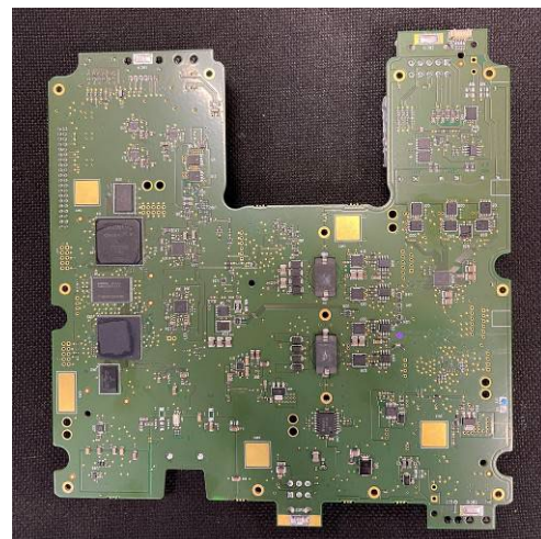
CPU PCBA - underside
