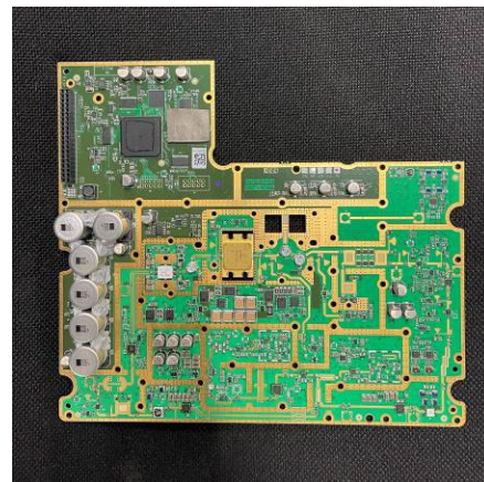
RF PCBA - underside
