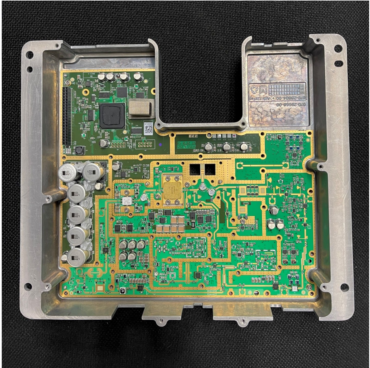
RF HOUSING + RF PCBA
