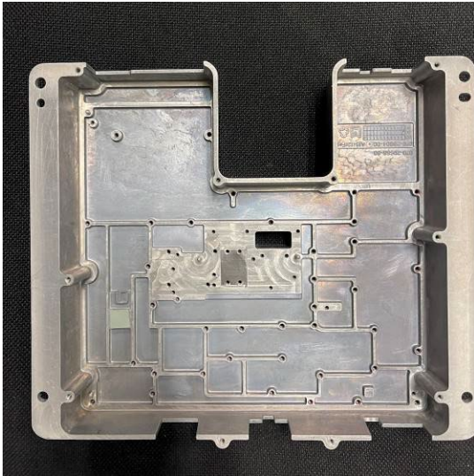
RF Housing - underside
