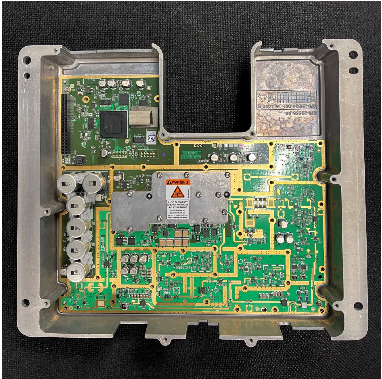
PA COVER OVER RF PCBA
