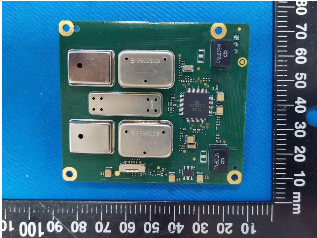
AIS Board
