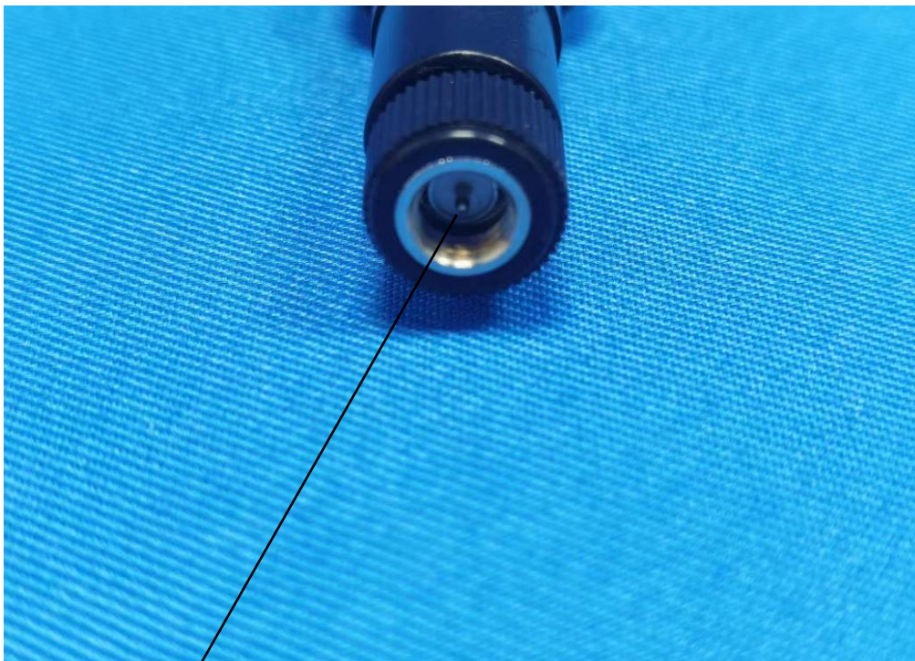
Reverse polarity types of antenna connector
