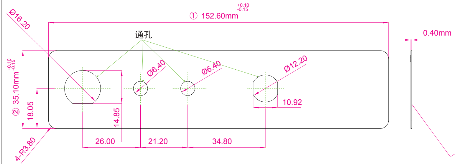
(Dimensional Drawing)
