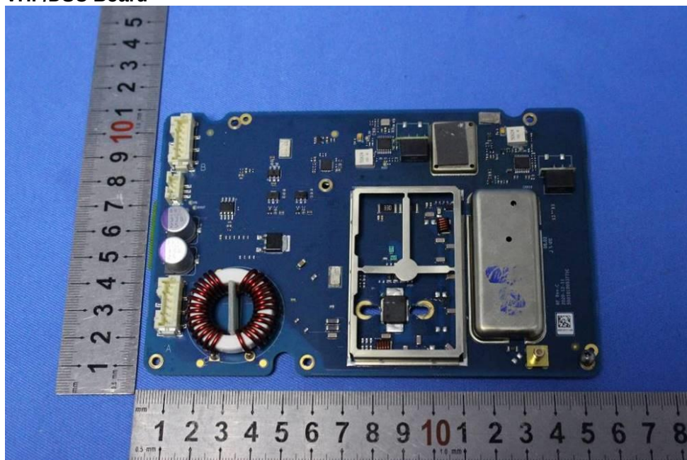
VHF/DSC Board
