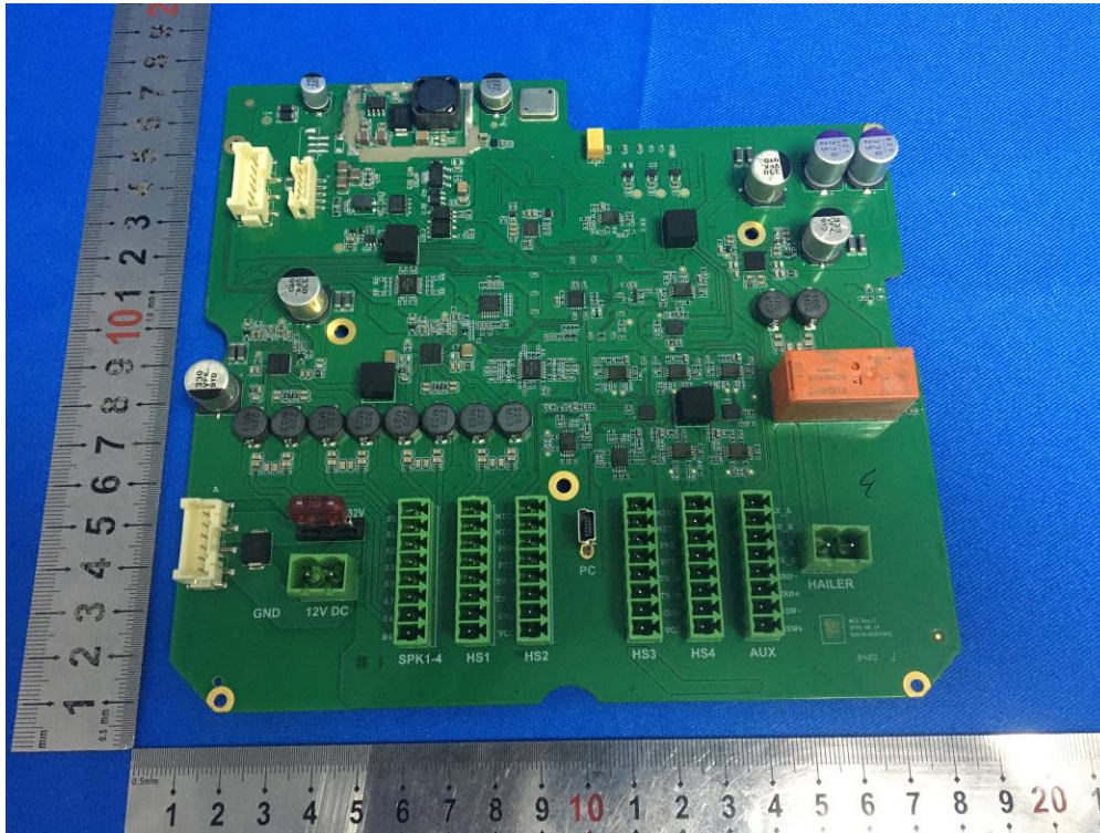
VHF/DSC Board
