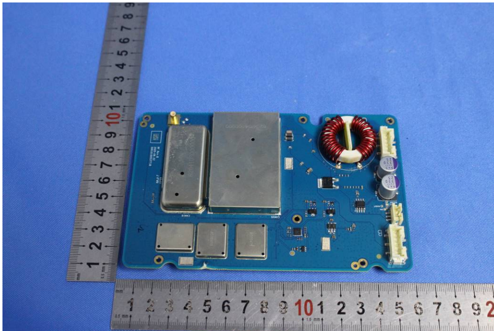
VHF/DSC Board
