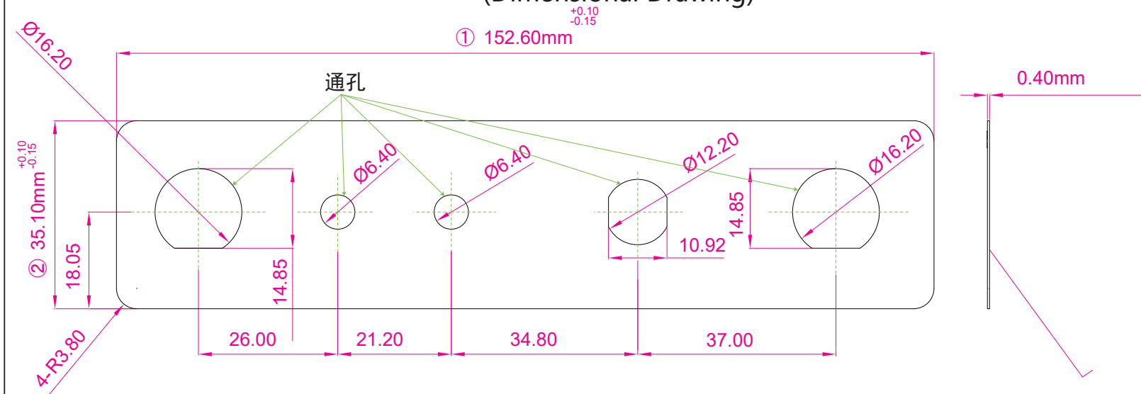
(Dimensional Drawing)
