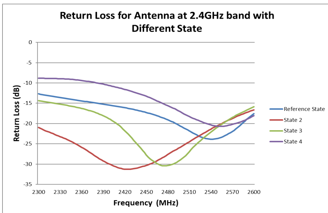
FIGURE 5.1.1 RETURN LOSS OF ANTENNA AT 2.4GHZ BAND WITH DIFFERENT STATE
