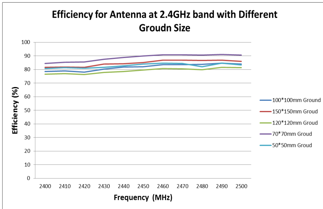
FIGURE 5.2.3 EFFICIENCY OF ANTENNA AT 2.4GHZ BAND WITH DIFFERENT GROUND SIZE
