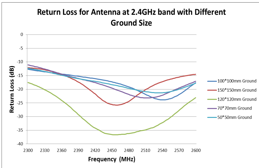
FIGURE 5.2.1 RETURN LOSS OF ANTENNA AT 2.4GHZ BAND WITH DIFFERENT GROUND SIZE
