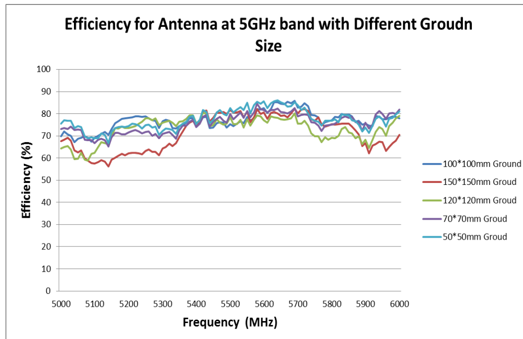
FIGURE 5.2.4 EFFICIENCY OF ANTENNA AT 5GHZ BAND WITH DIFFERENT GROUND SIZE
