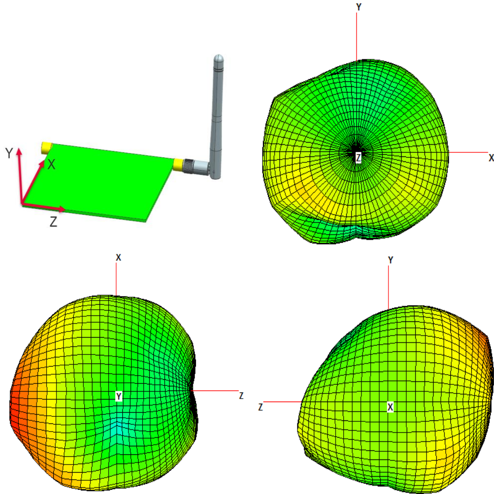
FIGURE 4.5.3 3D RADIATION PATTERN OF ANTENNA AT 2450MHZ IN FREE SPACE
