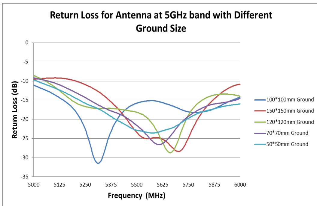
FIGURE 5.2.2 RETURN LOSS OF ANTENNA AT 5GHZ BAND WITH DIFFERENT GROUND SIZE
