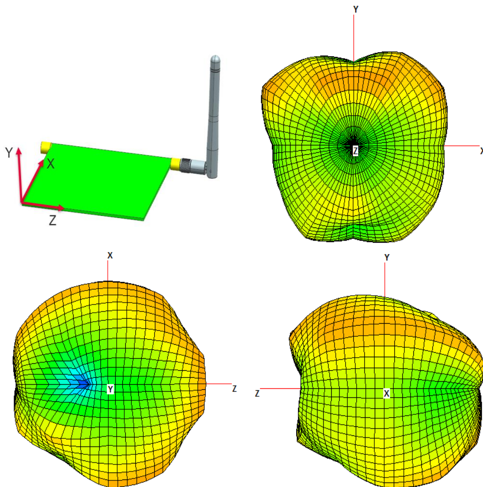
FIGURE 4.5.4 3D RADIATION PATTERN OF ANTENNA AT 5500MHZ IN FREE SPACE
