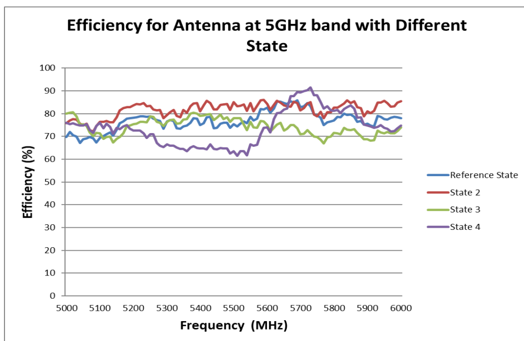
FIGURE 5.1.4 EFFICIENCY OF ANTENNA AT 5GHZ BAND WITH DIFFERENT STATE
