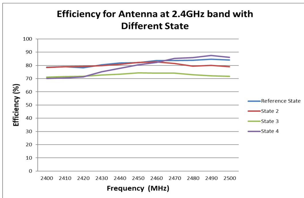
FIGURE 5.1.3 EFFICIENCY OF ANTENNA AT 2.4GHZ BAND WITH DIFFERENT STATE
