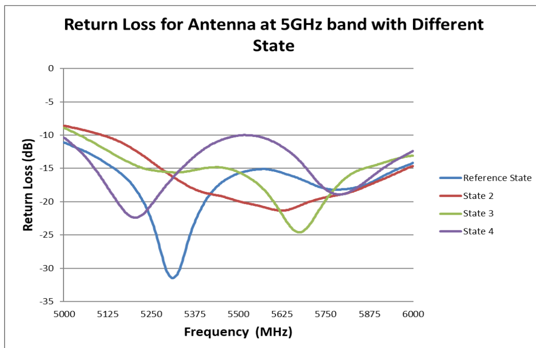
FIGURE 5.1.2 RETURN LOSS OF ANTENNA AT 5GHZ BAND WITH DIFFERENT STATE
