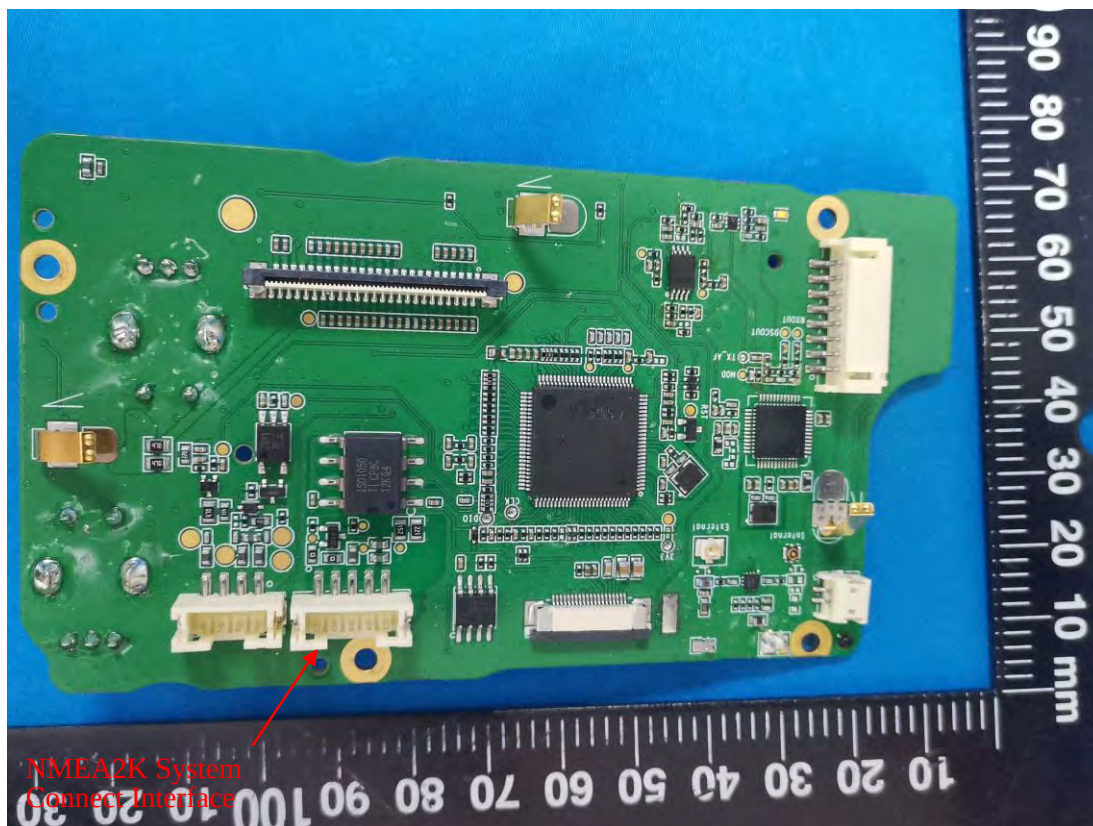
MCU Board
