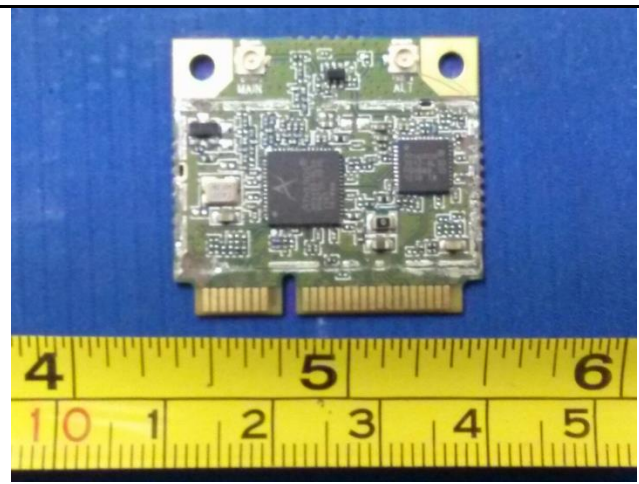
Radio Board – Top View without Shielding
