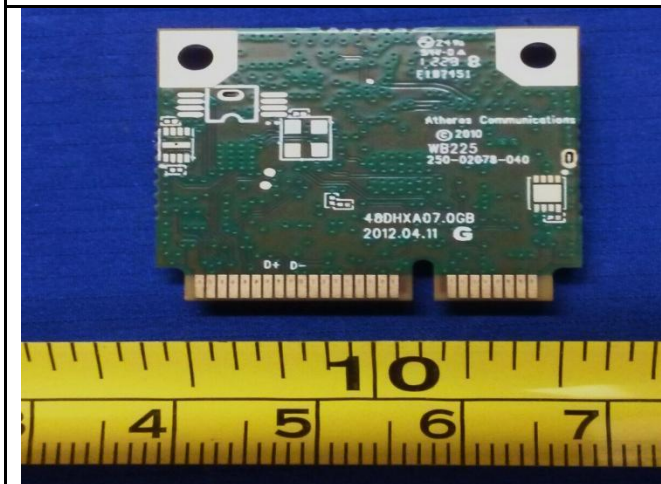
Radio Board – Bottom View
