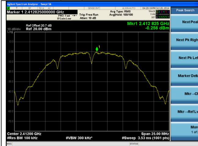
PSD-2.4G-802.11b Low
