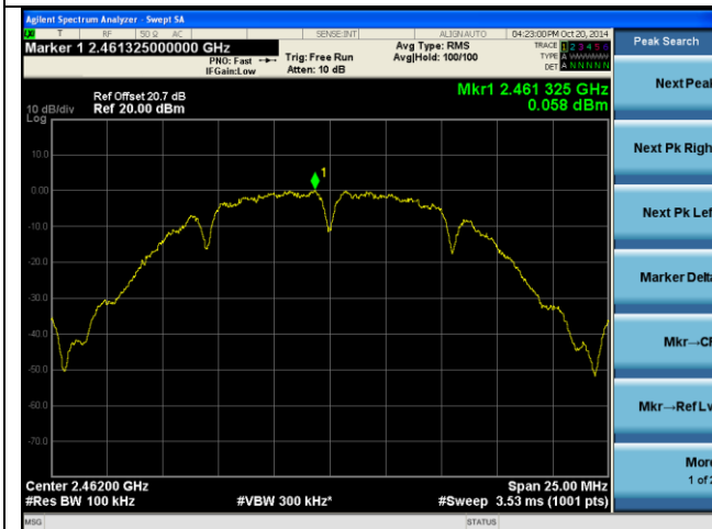
PSD-2.4G-802.11b High
