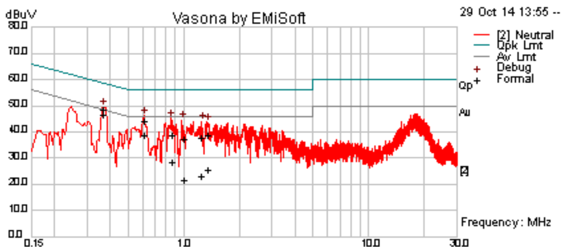
Neutral Line Plot @ 120Vac, 60Hz
