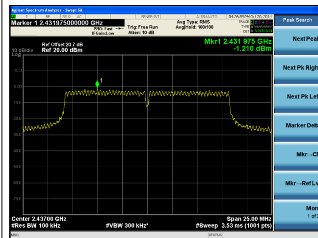
PSD-2.4G-802.11g Mid
