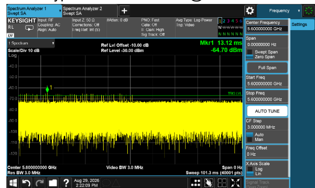
Radar Type 1 Calibration Plot @5600MHz
