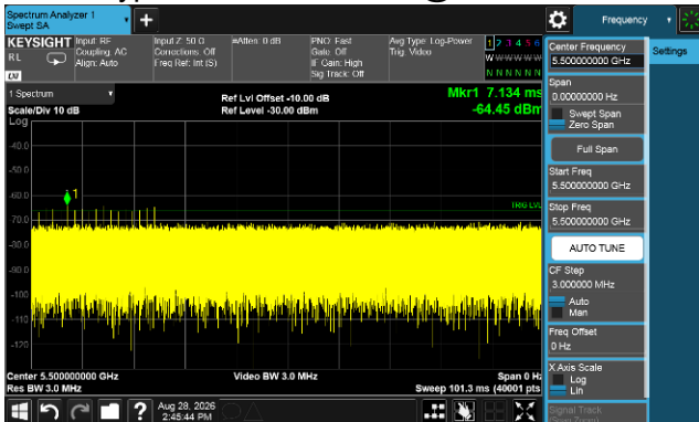
Radar Type 0 Calibration Plot @5500MHz
