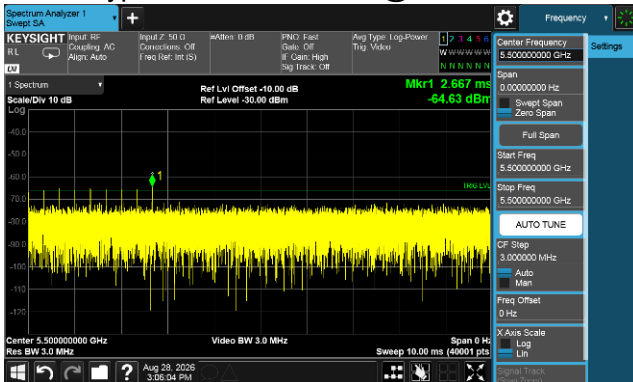
Radar Type 6 Calibration Plot @5500MHz
