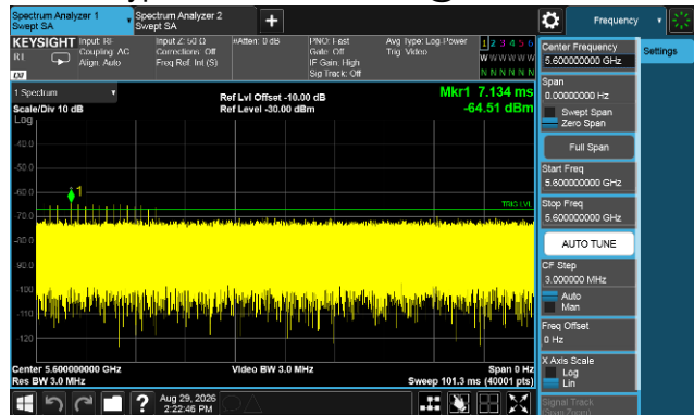
Radar Type 0 Calibration Plot @5600MHz
