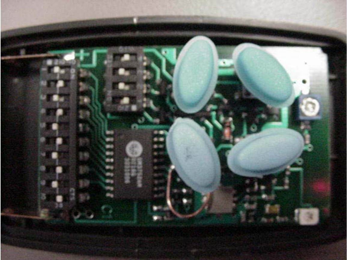
Circuit Card – Top Side
