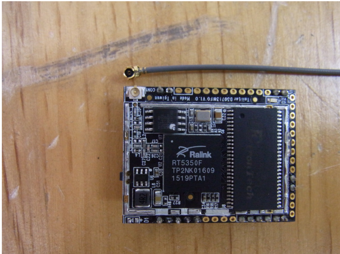
Antenna Port
