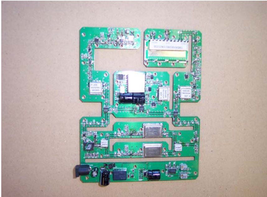
EUT – Downlink Component with Shield View
