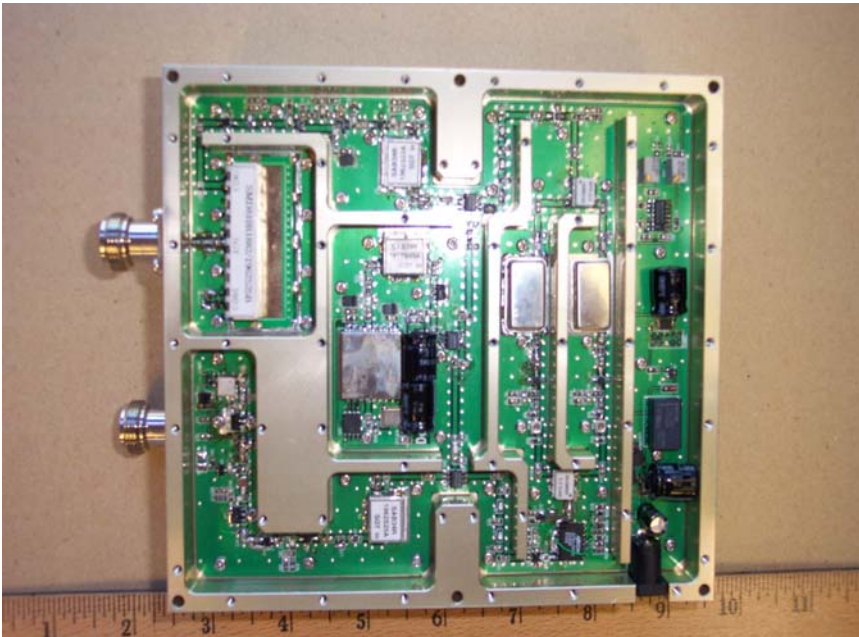
EUT – Downlink Component with Shield View
