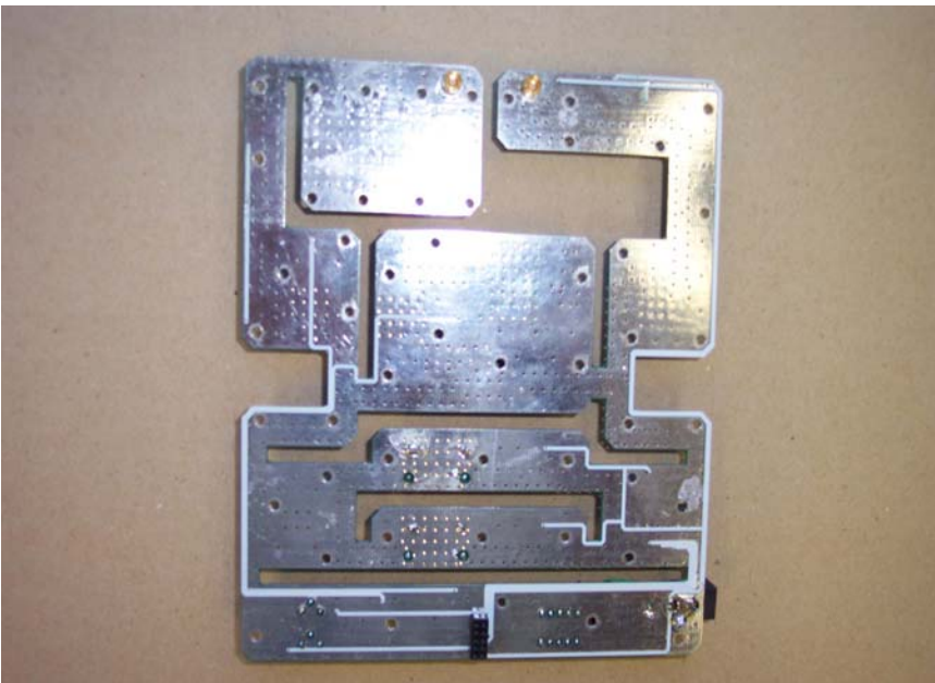
EUT – Downlink Solder View
