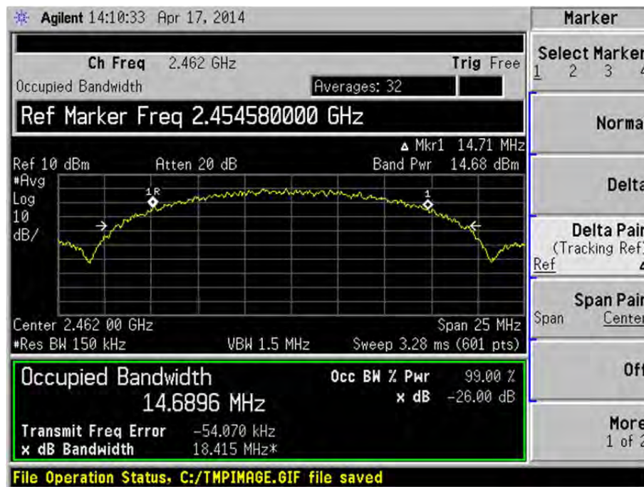
802.11 b (Channel 11)
