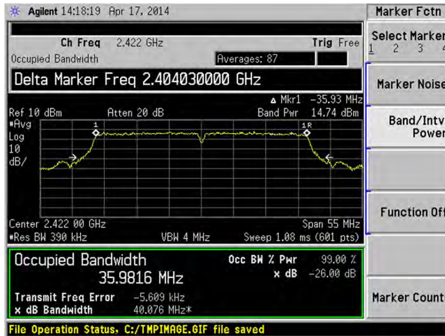
802.11 n-HT40 (Channel 3)
