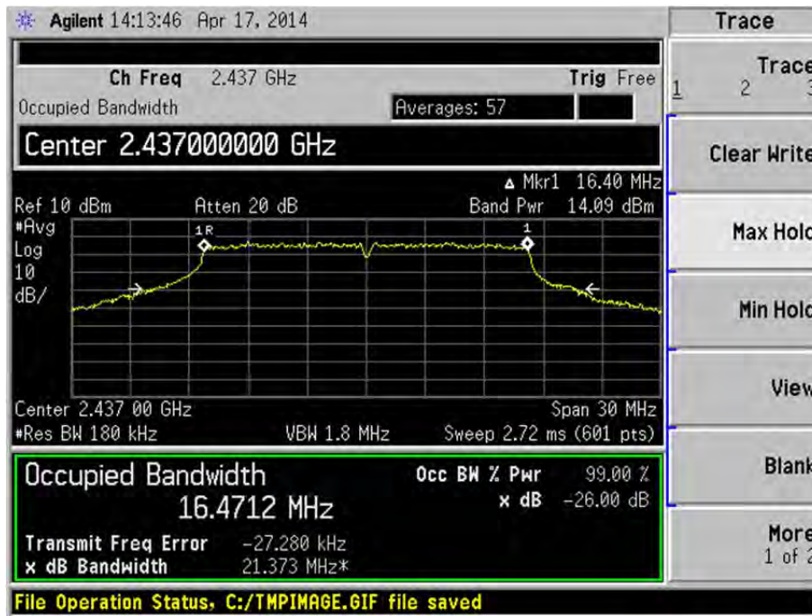
802.11 g (Channel 6)
