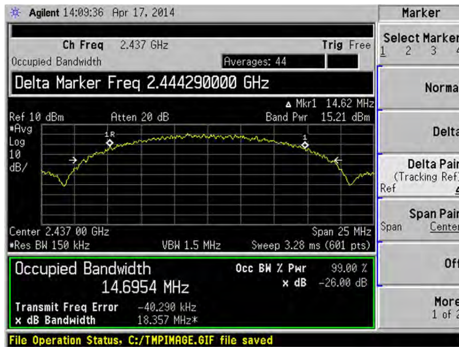
802.11 b (Channel 6)
