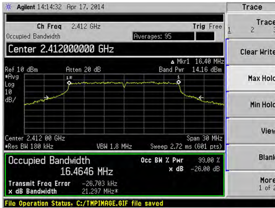
802.11 g (Channel 1)
