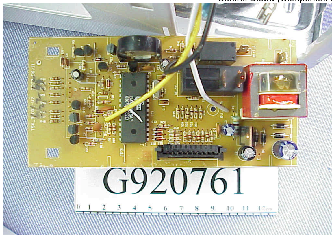
Control Board (Component Side)
