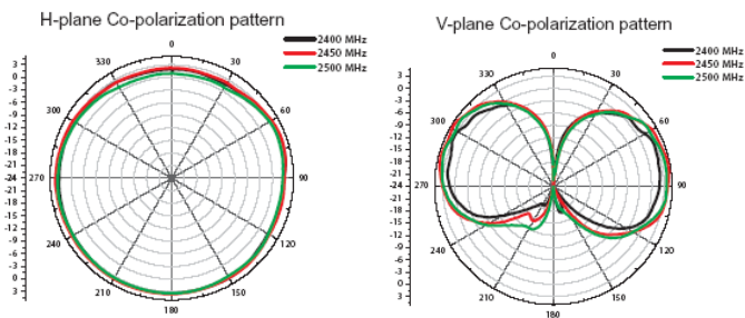
Figure 4 Co-polarization Pattern
