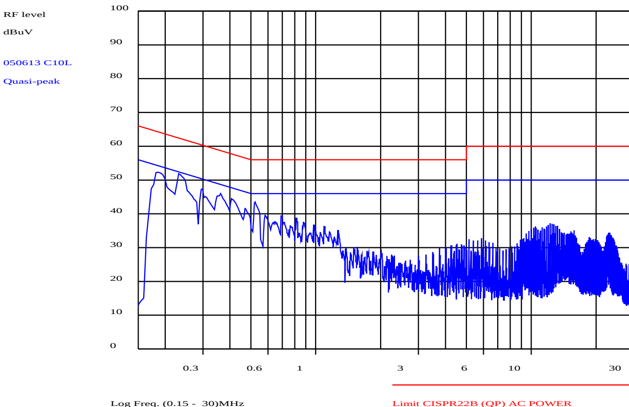
PLOT 2 Conducted Emissions - Live Line - 115V
