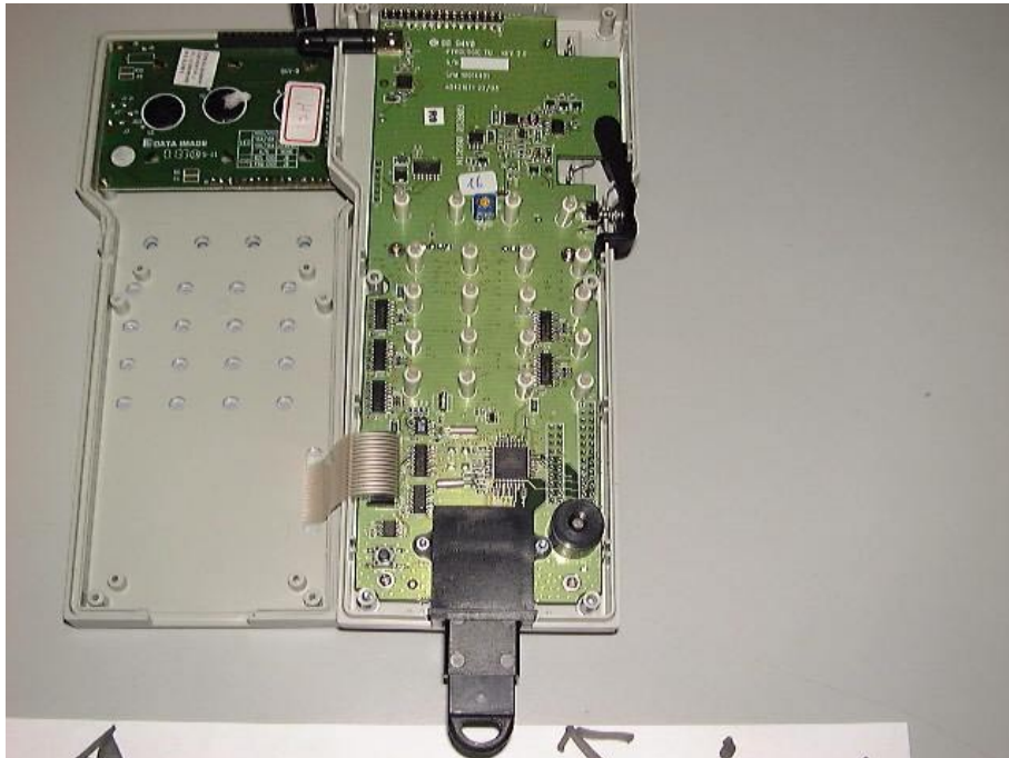
Figure 2 Top View Cover Removed
