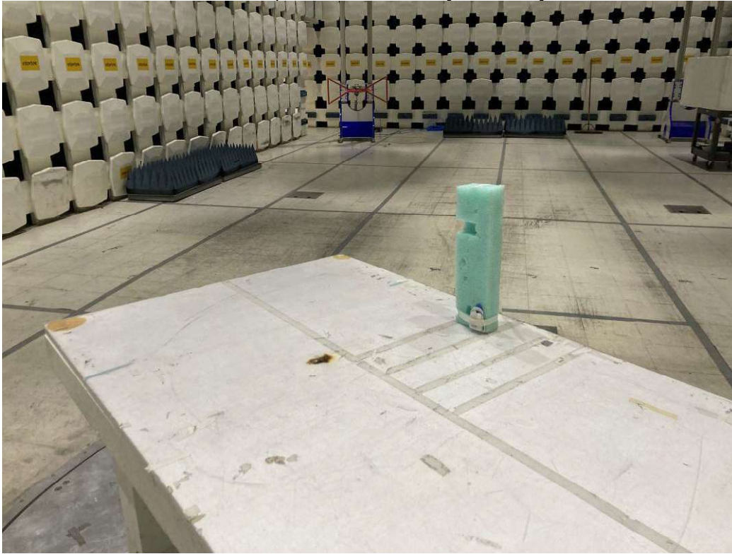
Test Setup, RE 30-1000 MHz [Short Side]
