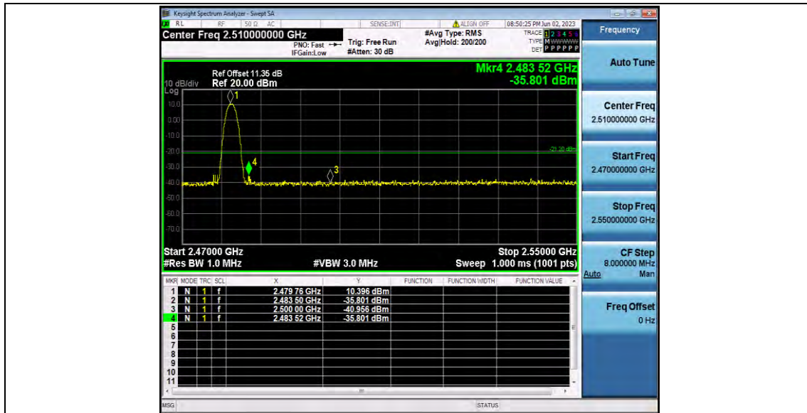
2DH1_Ant1_High_2480_Peak
