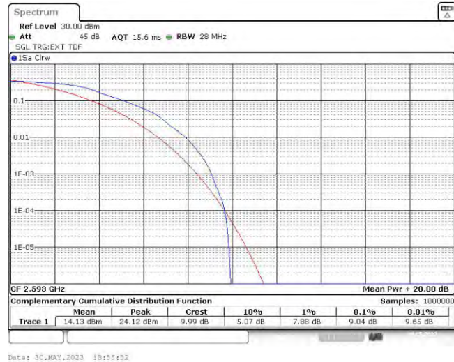
Band41-20MHz-QPSK-40620-100RB#0
