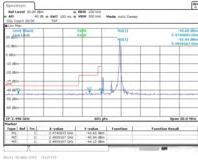
Band41-5MHz-16QAM-39675-25RB#0
