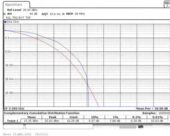
Band41-15MHz-QPSK-40620-75RB#0
