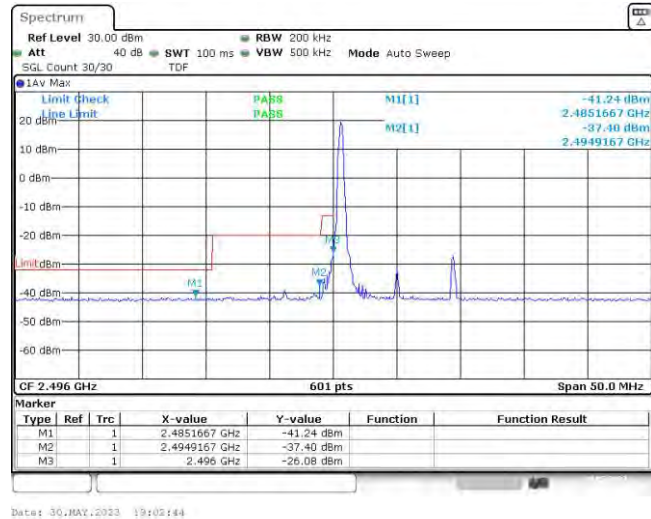
Band41-10MHz-QPSK-39700-1RB#49
