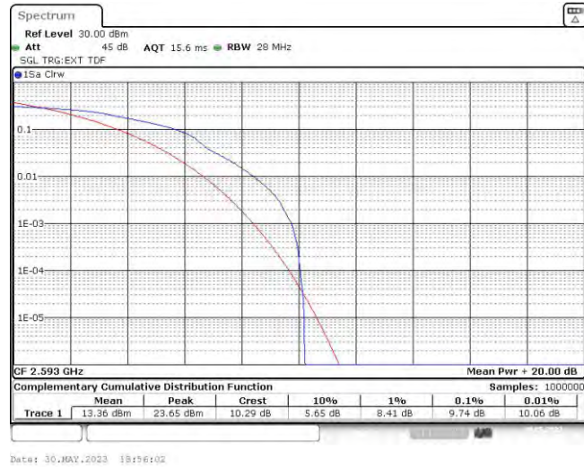
Band41-20MHz-16QAM-40620-100RB#0
