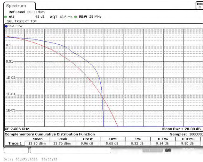
Band41-20MHz-16QAM-39750-100RB#0
