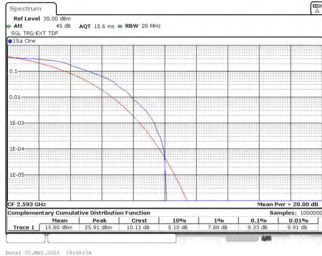
Band41-10MHz-QPSK-40620-50RB#0
