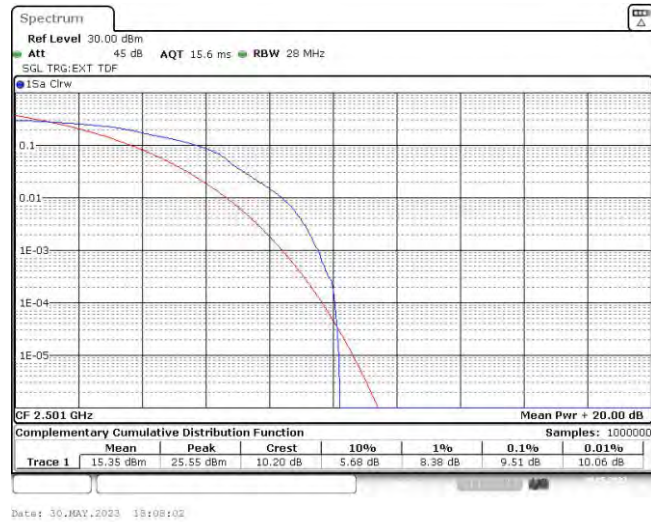
Band41-10MHz-16QAM-39700-50RB#0
