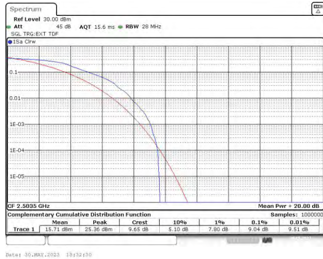
Band41-15MHz-QPSK-39725-75RB#0
