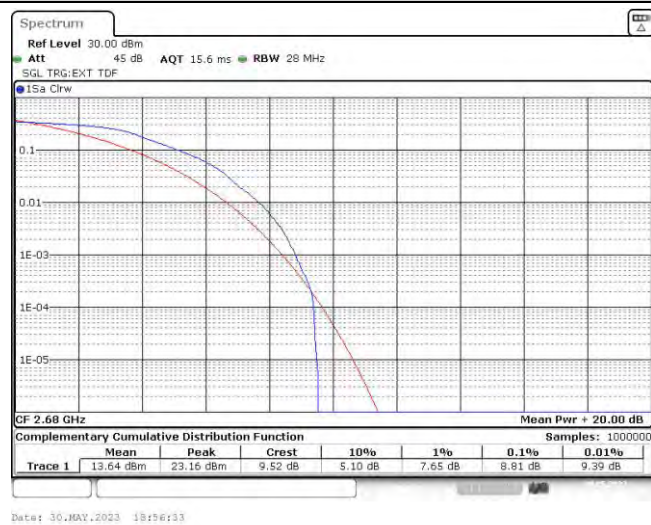
Band41-20MHz-QPSK-41490-100RB#0
