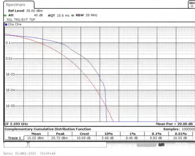
Band41-10MHz-16QAM-40620-50RB#0
