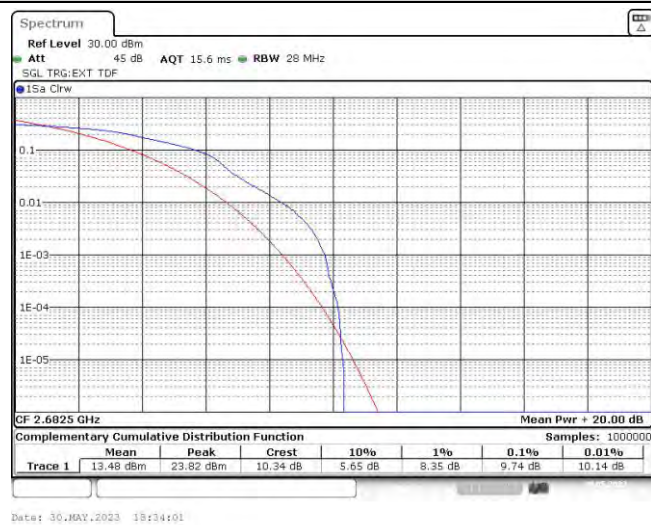
Band41-15MHz-16QAM-41515-75RB#0
