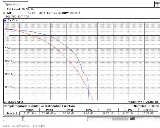
Band41-5MHz-16QAM-40620-25RB#0
