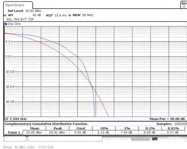
Band41-5MHz-QPSK-40620-25RB#0
