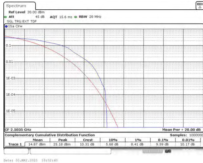
Band41-15MHz-16QAM-39725-75RB#0
