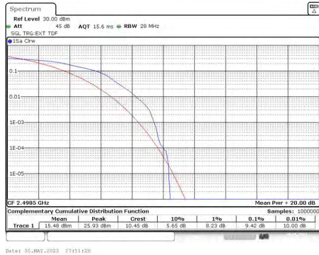
Band41-5MHz-16QAM-39675-25RB#0
