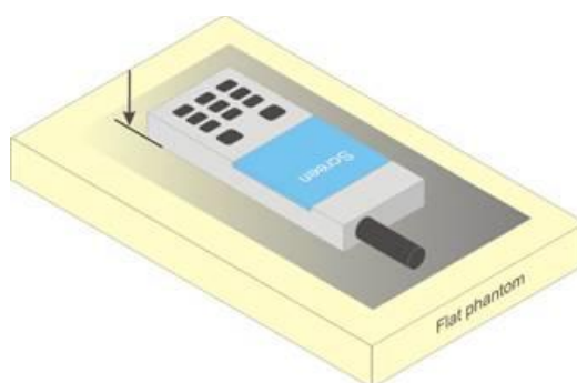
F-3.Test positions for hand-held devices
