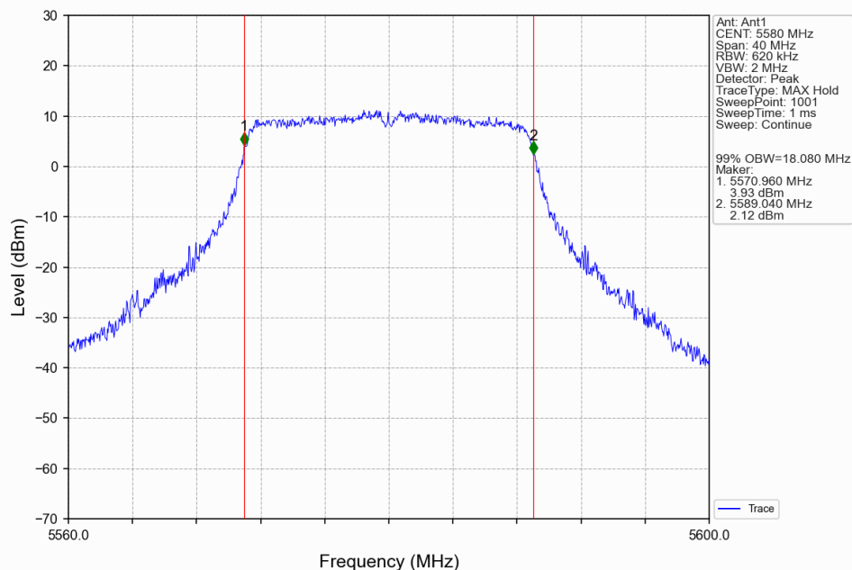
802.11ac(VHT20)_MCH_5580MHz_Ant1_NTNV
