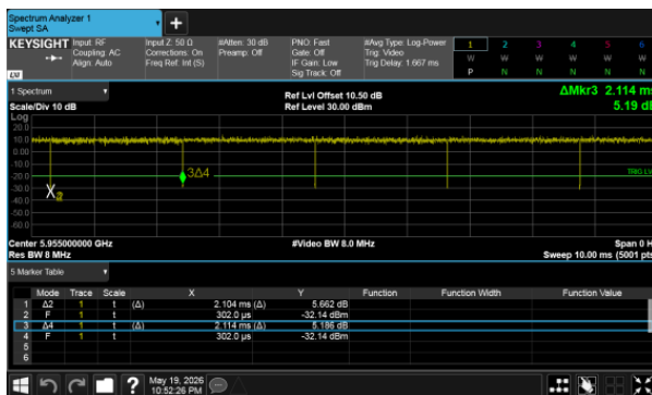
Modulation Type: 802.11ax HE20
