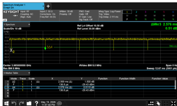
Modulation Type: 802.11ax HE160
