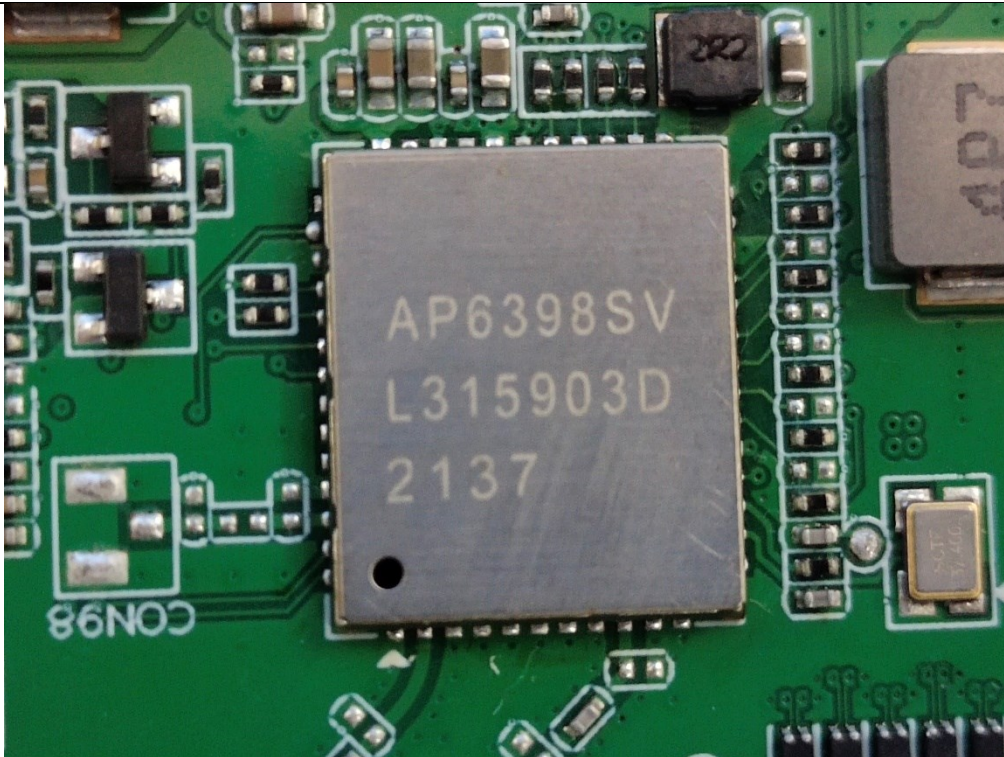
(4) EUT Photo ( ESY10I4 )
