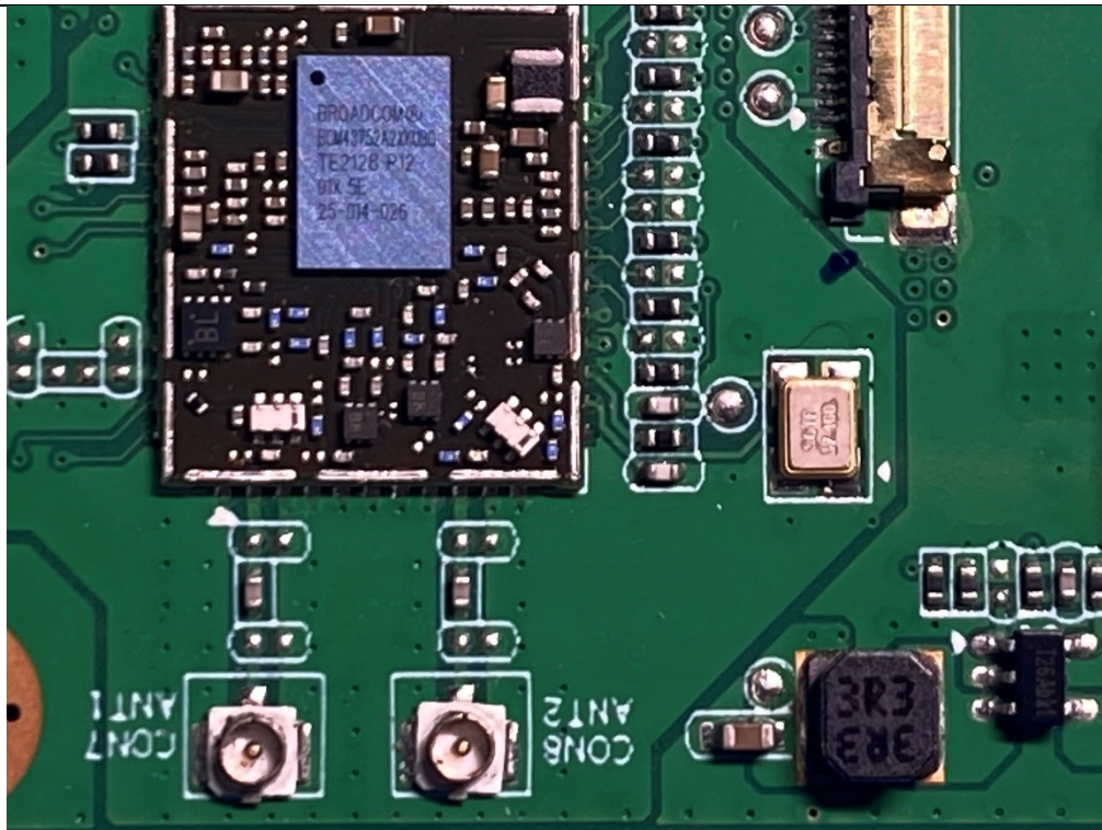
(12) EUT Photo ( ESY15I4-C )
