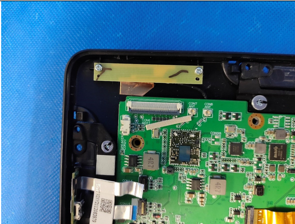
(8) EUT Photo ( ESY15I4-C )
