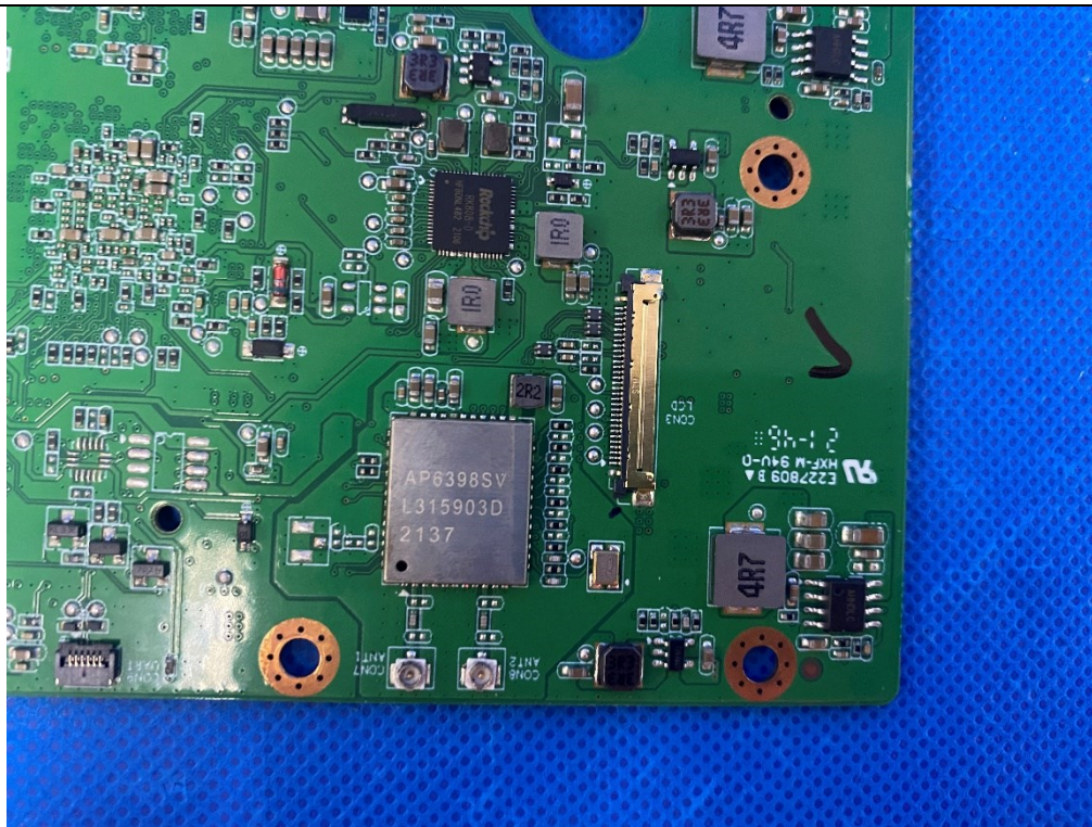
(11) EUT Photo ( ESY15I4-C )
