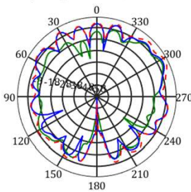
frequency=5150MHz, Y-Z Plane
