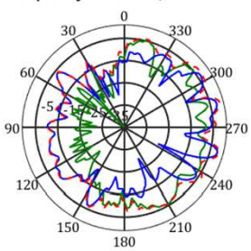
frequency=5470MHz, X-Y Plane
