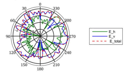
frequency=6125MHz, X-Y Plane
