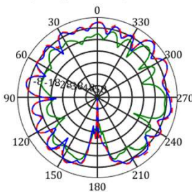
frequency=5850MHz, Y-Z Plane
