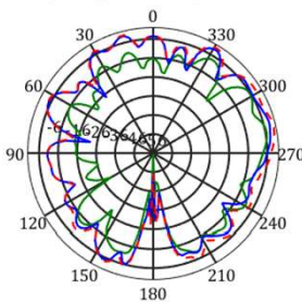
frequency=5470MHz, Y-Z Plane
