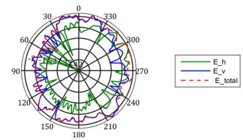
frequency=6525MHz, X-Y Plane
