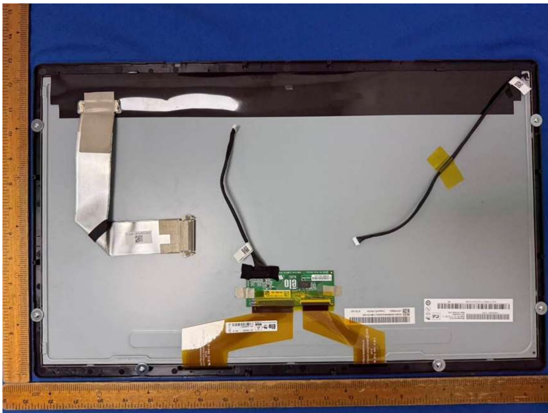
Panel Brand: AUO,Model: M215HAN01.2
