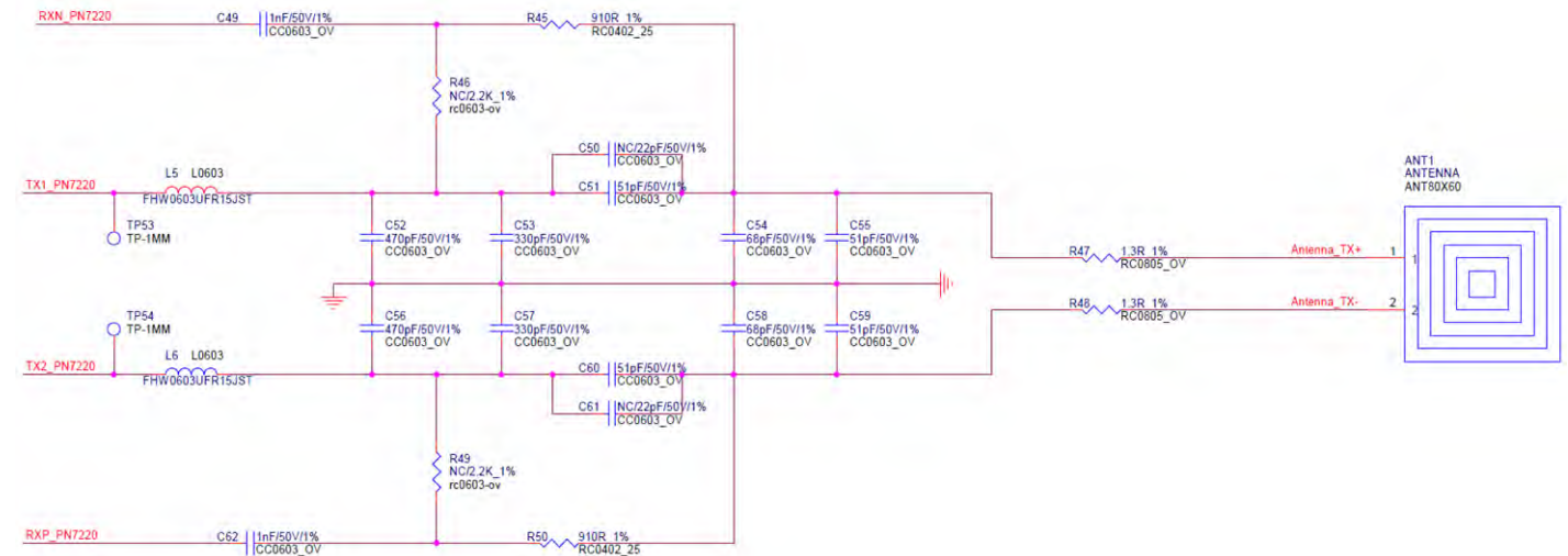
ANTENNA Interfacing
