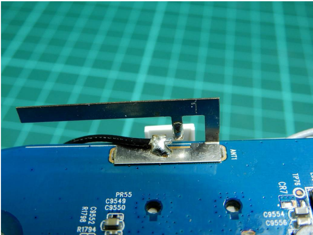
(42) EUT Photo (2.4GHz WLAN Antenna)
