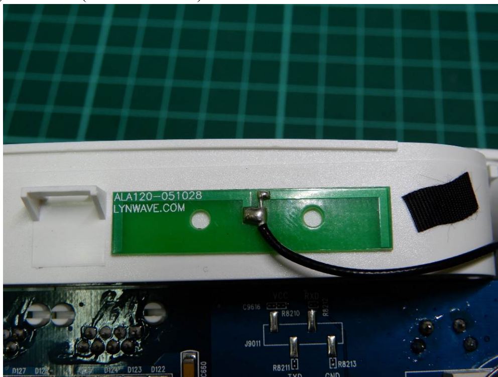
(54) EUT Photo (Bluetooth Antenna)
