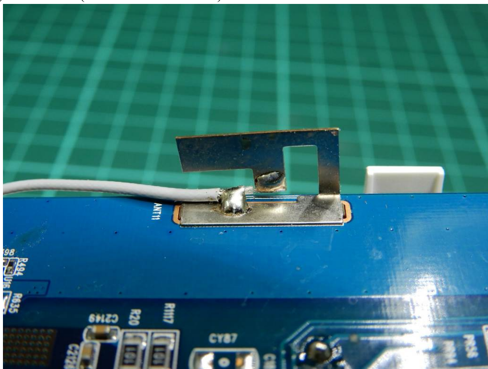
(44) EUT Photo (5GHz WLAN Antenna)
