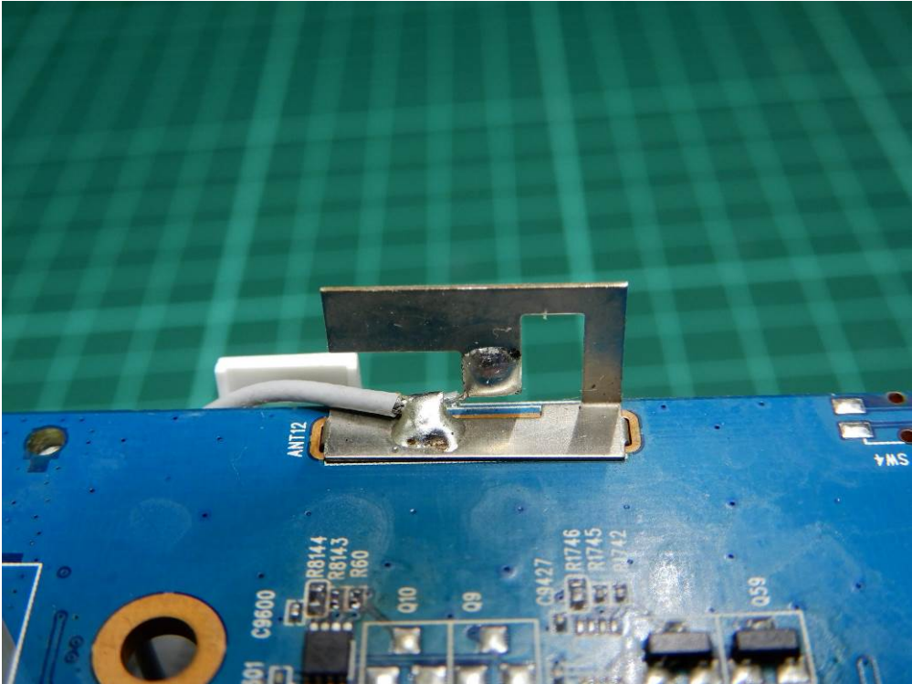
(45) EUT Photo (5GHz WLAN Antenna)
