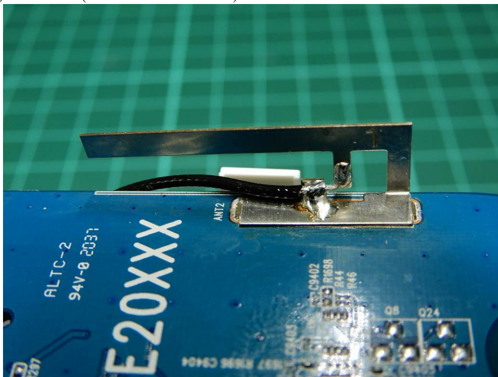
(43) EUT Photo (2.4GHz WLAN Antenna)
