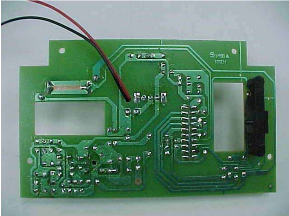
RCB96849_PCB2 (640x480x16M jpeg)
