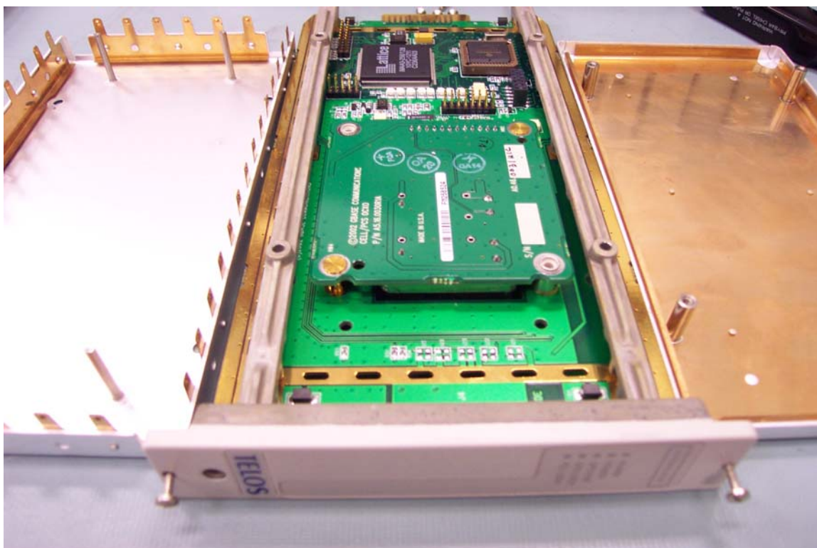
Timing Card – bottom
