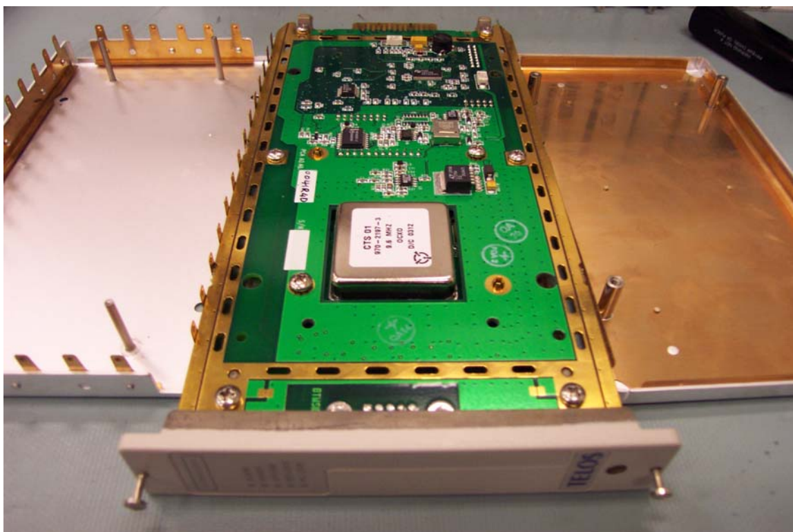
Timing Card – top
