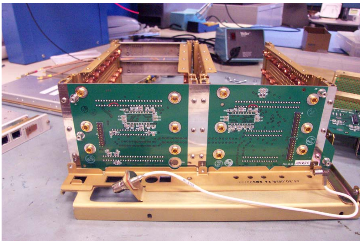
Back Backplane Board
