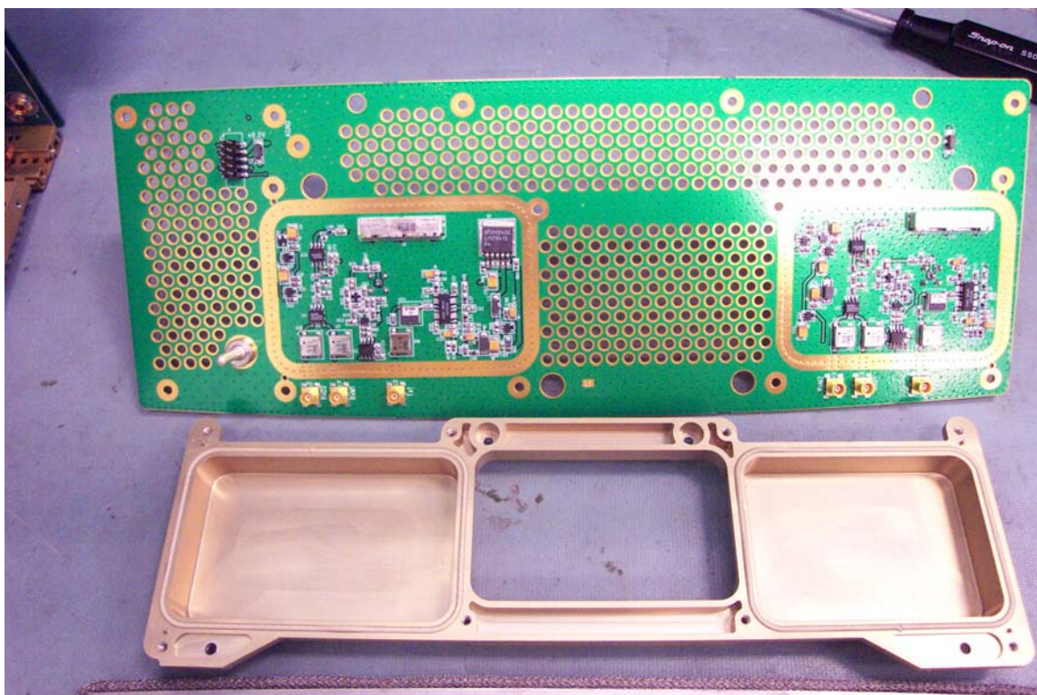
Front RFS – no shield
