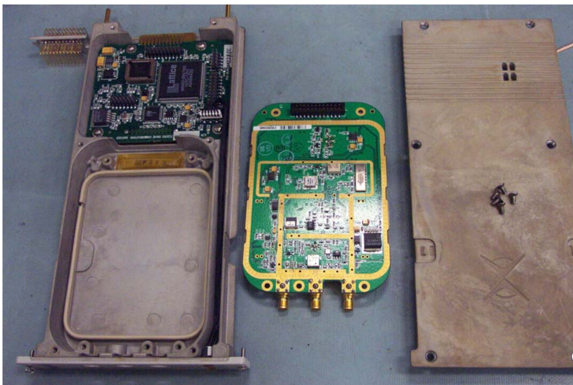
PCS RFM & Digitizer without shield
