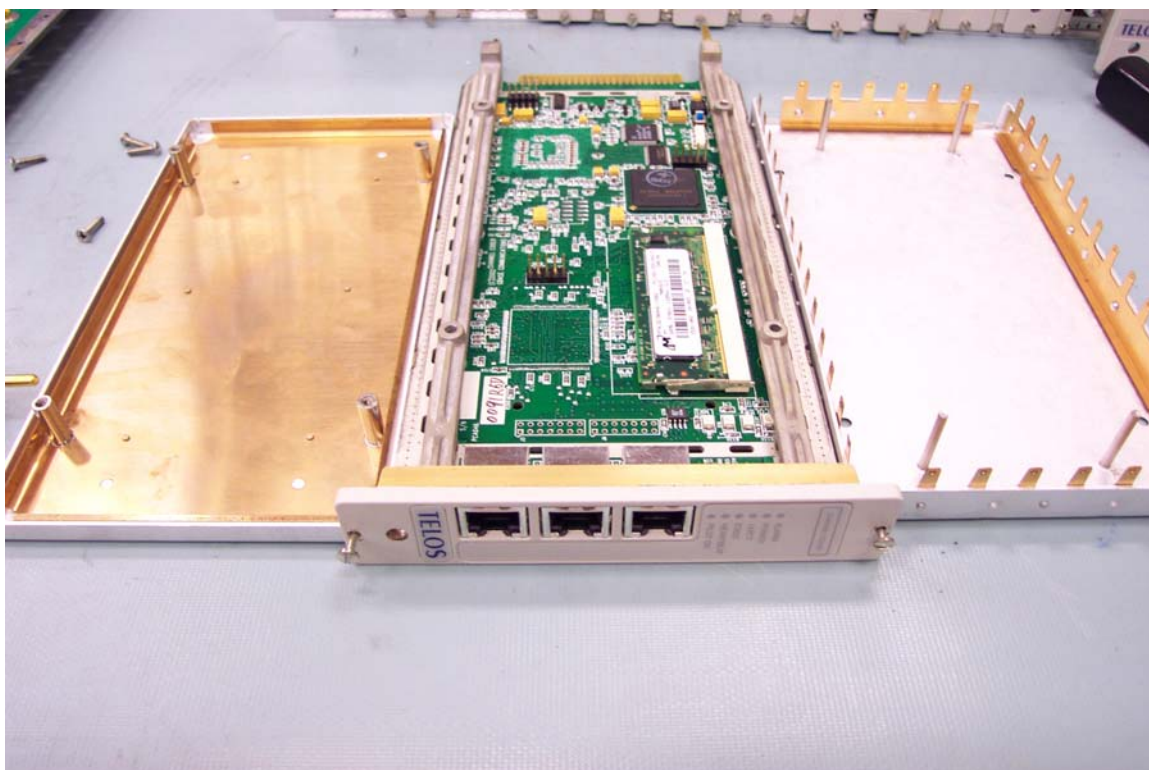
Channel Card top
