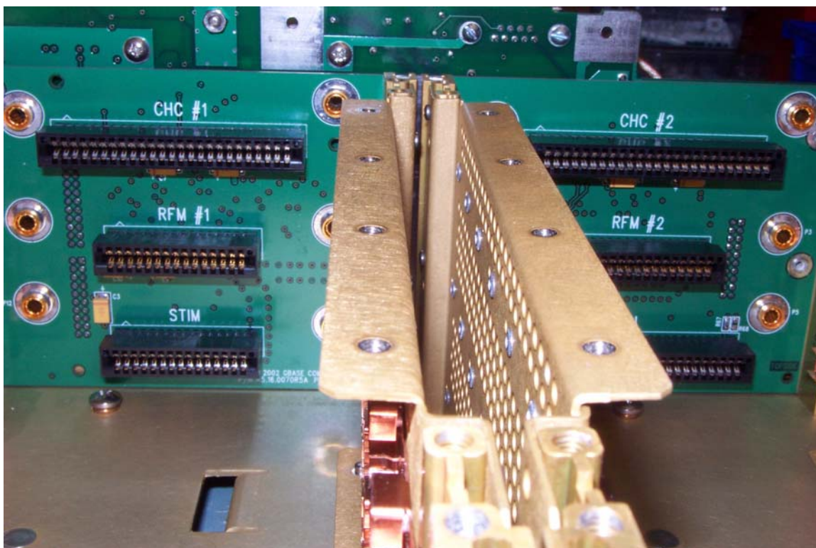
Front Backplane Board
