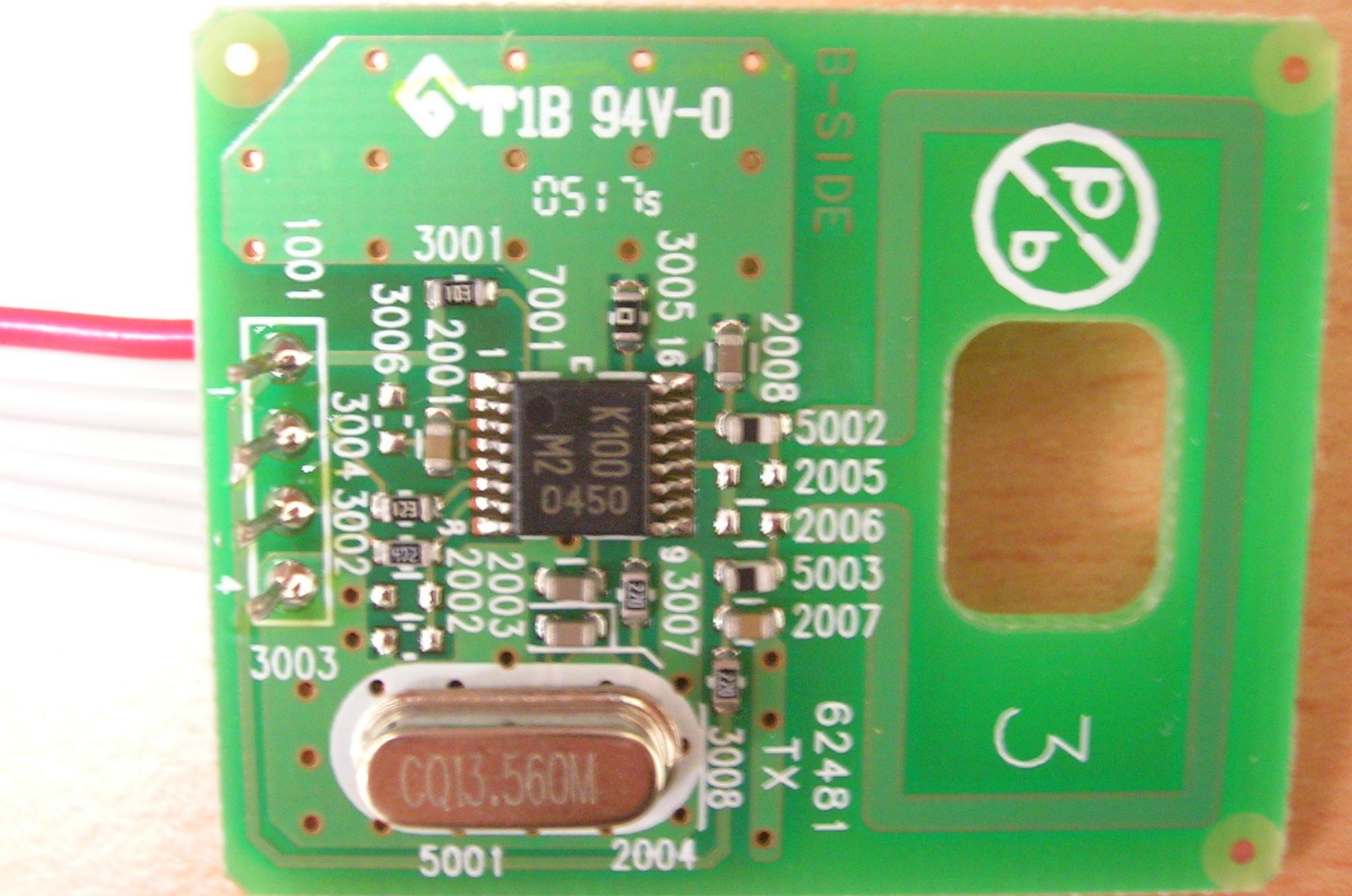
Sub PCB Front Photo
