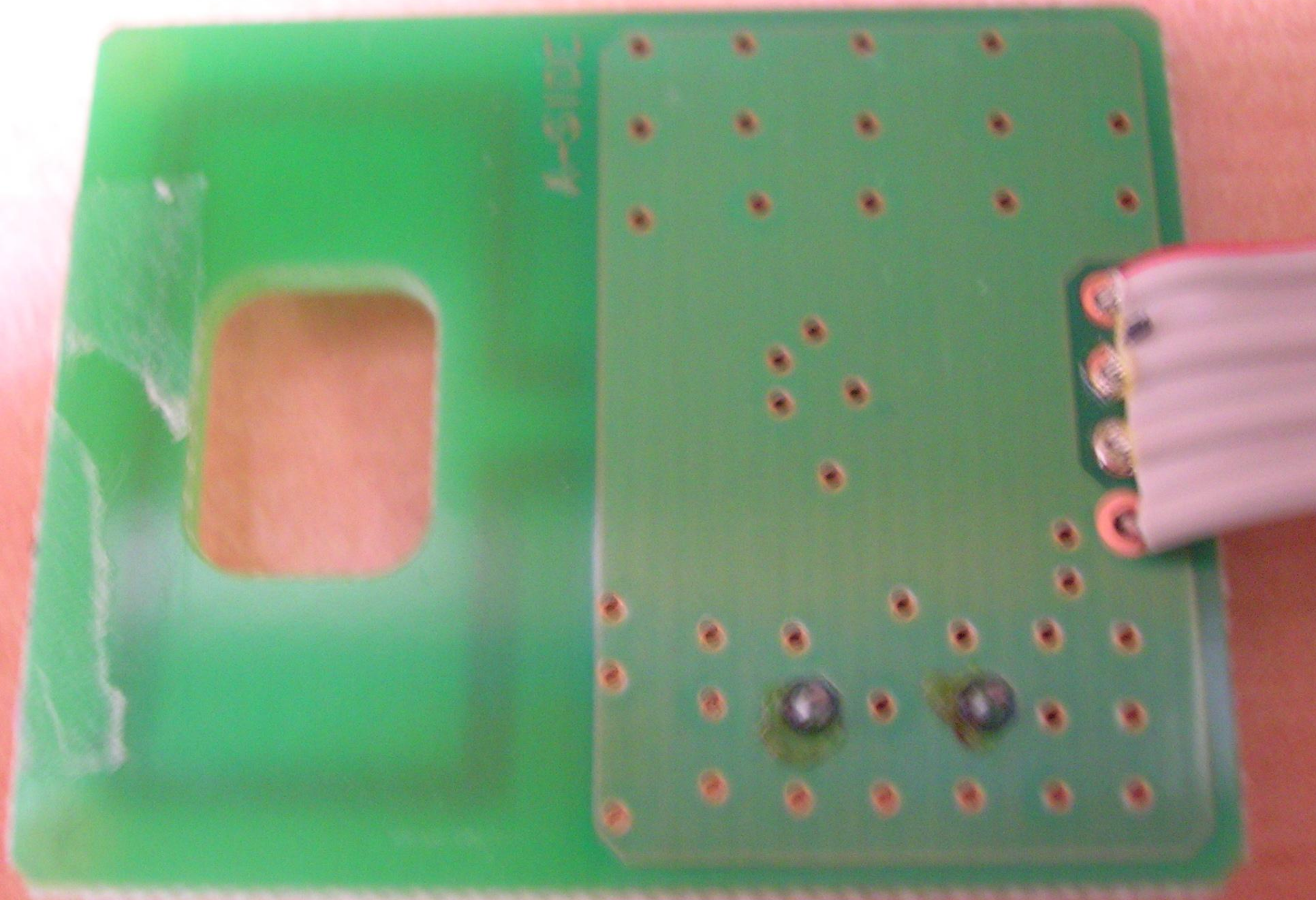
Sub PCB Rear Photo
