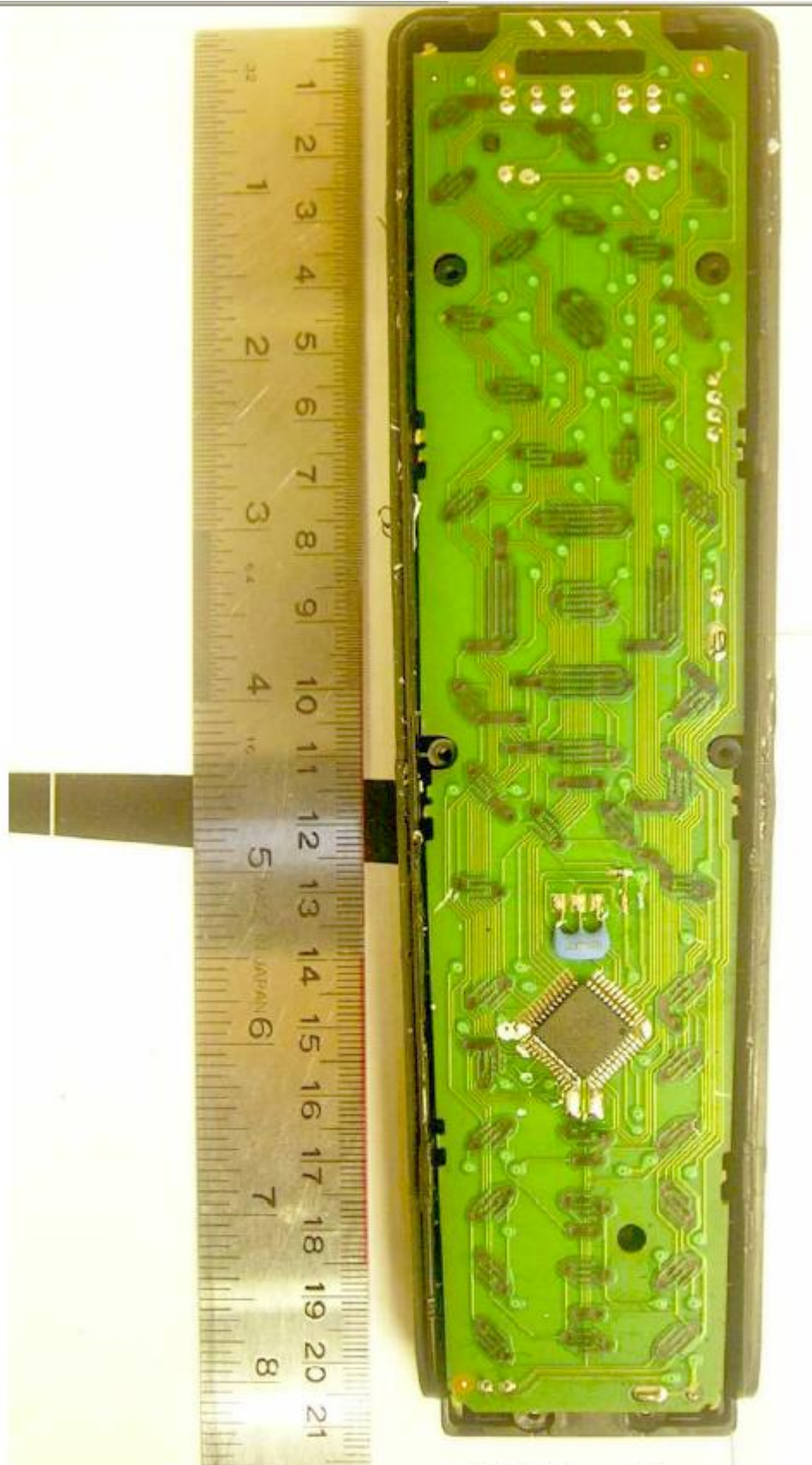
EUT Internal View
