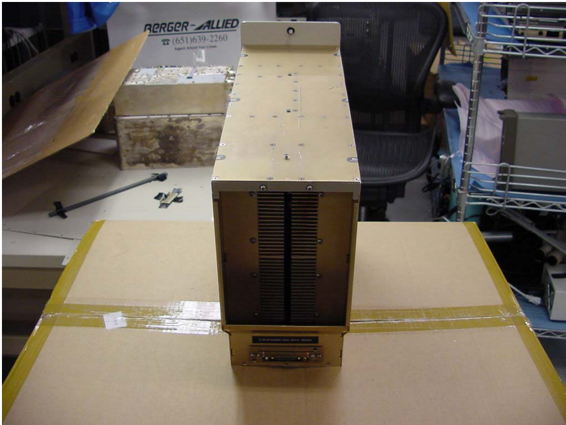
Figure 3 LPA Rear View
