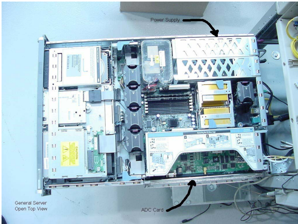
Figure 5 Server Open Top View
