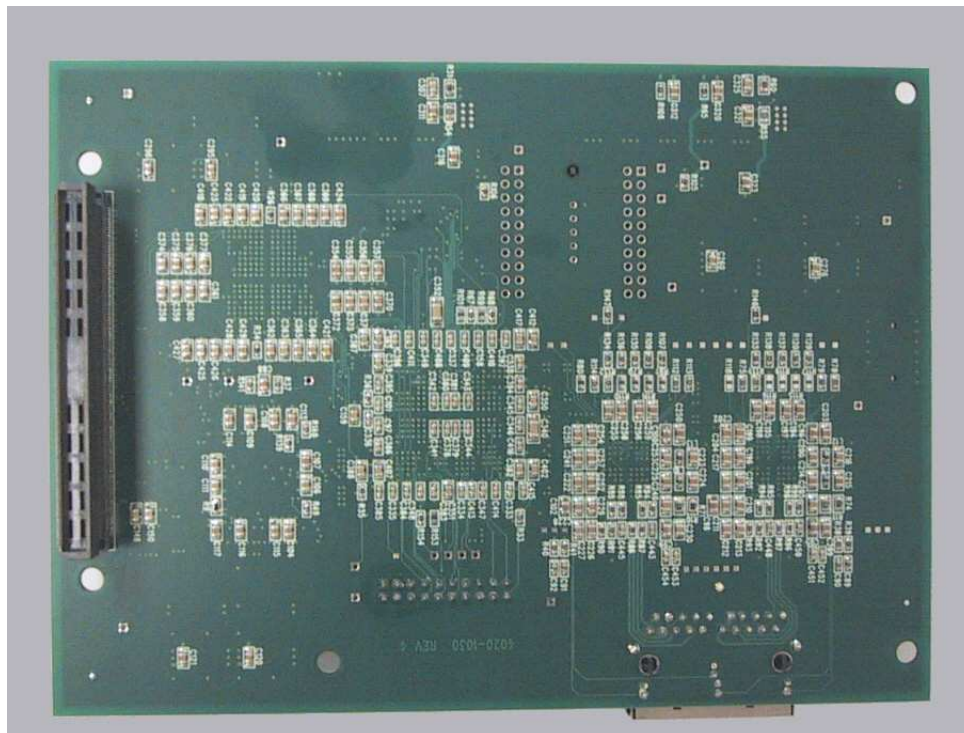
Figure 3 – Daughter Card - Back
