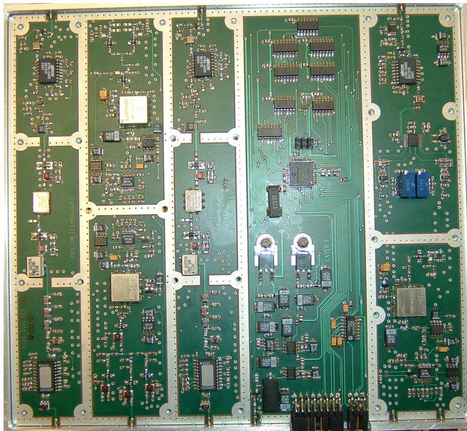
Figure 6 – RF Board Front
