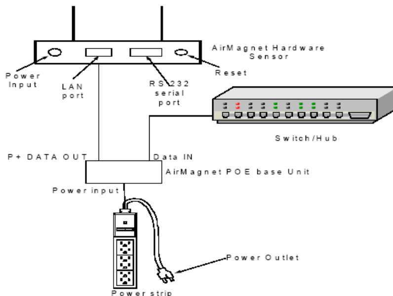
Figure 2: AirMagnet POE Injector
