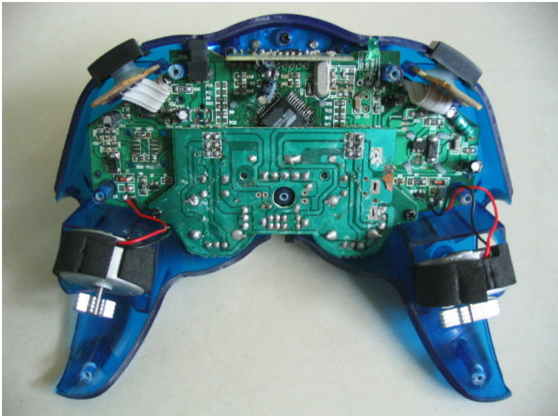
Internal of Game Pad-2
