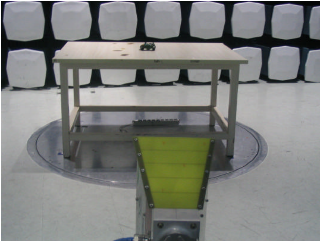
Setup Photo-4
