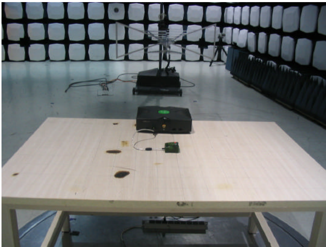
Setup Photo-4
