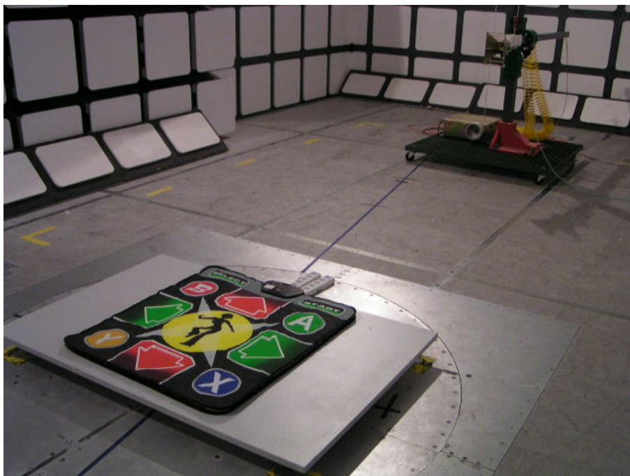
Above 1GHz:Radiated Emission - Rear View
