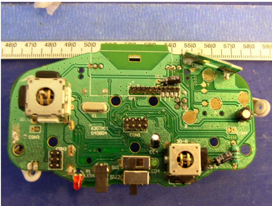
Transmitter Component View
