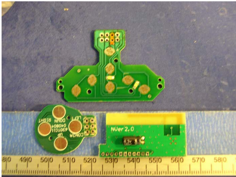
Transmitter Small PCB Front Component View
