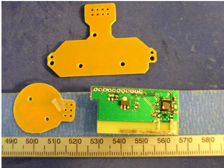
Transmitter Small PCB Rear Solder View
